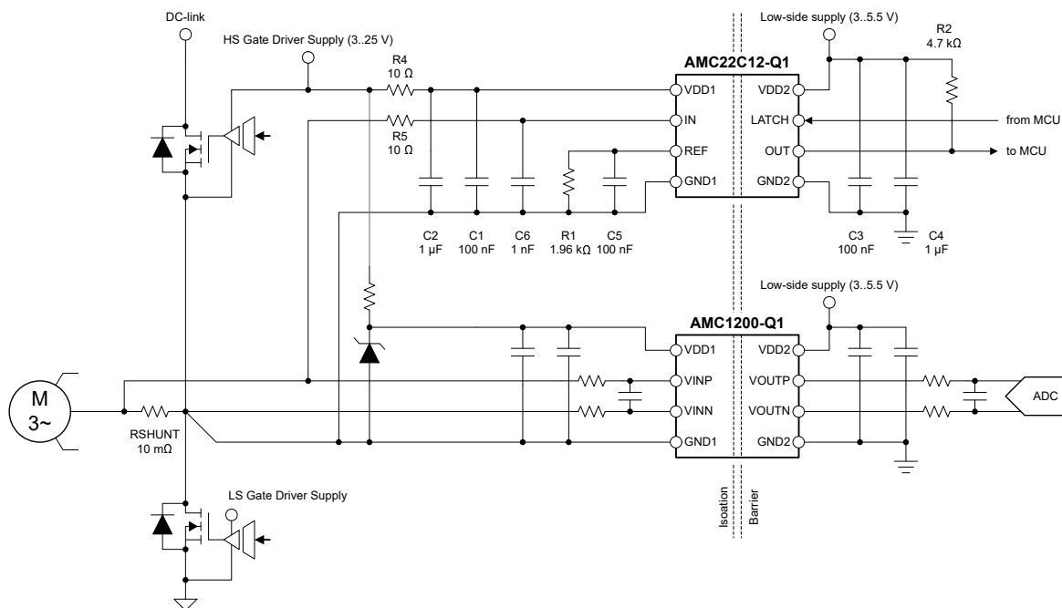
Figure 7-1. Using the AMC22C12-Q1 for Overcurrent Detection
