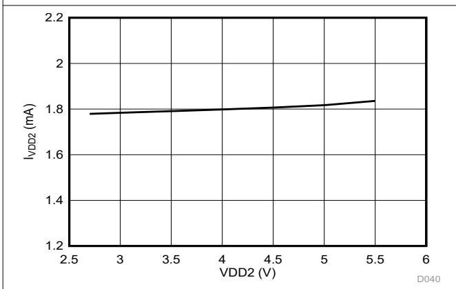
Figure 5-44. High-Side Supply Current vs Supply Voltage
