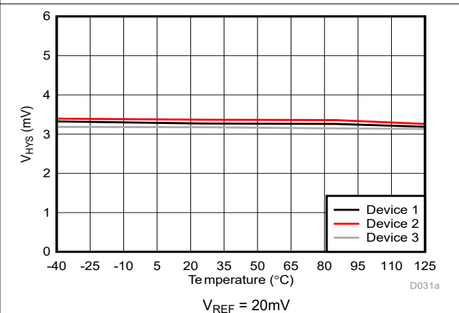
Figure 5-29. Cmp1 Trip Threshold Hysteresis vs Temperature
