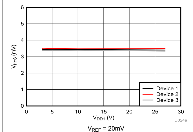
Figure 5-10. Cmp0 Trip Threshold Hysteresis vs Supply Voltage
