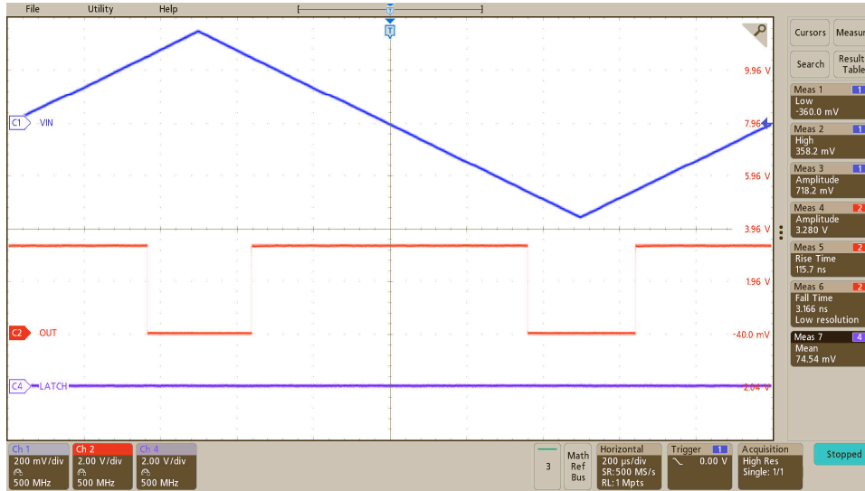
Figure 7-3. Output Response of the AMC22C12-Q1 to a Triangular Input Waveform
