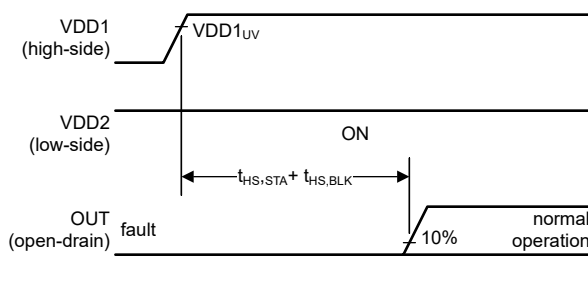
Figure 6-6. VDD2 is On; VDD1 Turns On (Long Delay)
