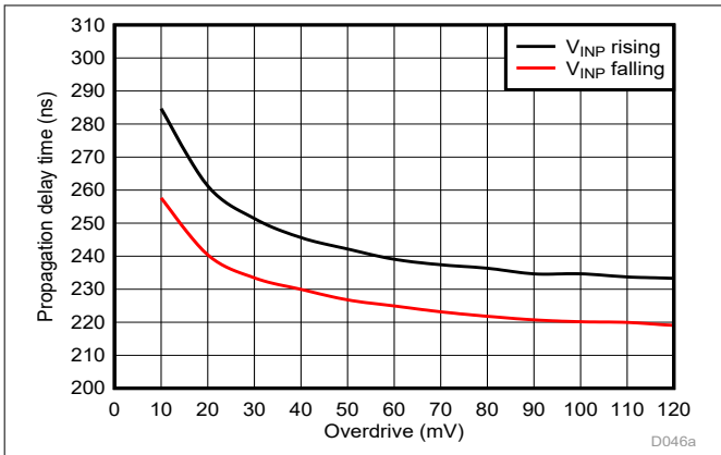
Figure 5-36. Cmp0 Propagation Delay vs Overdrive
