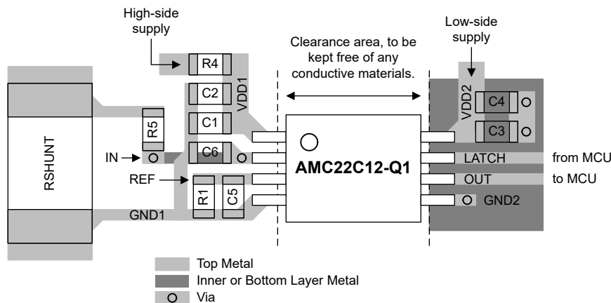
Figure 7-7. Recommended Layout of the AMC22C12-Q1
