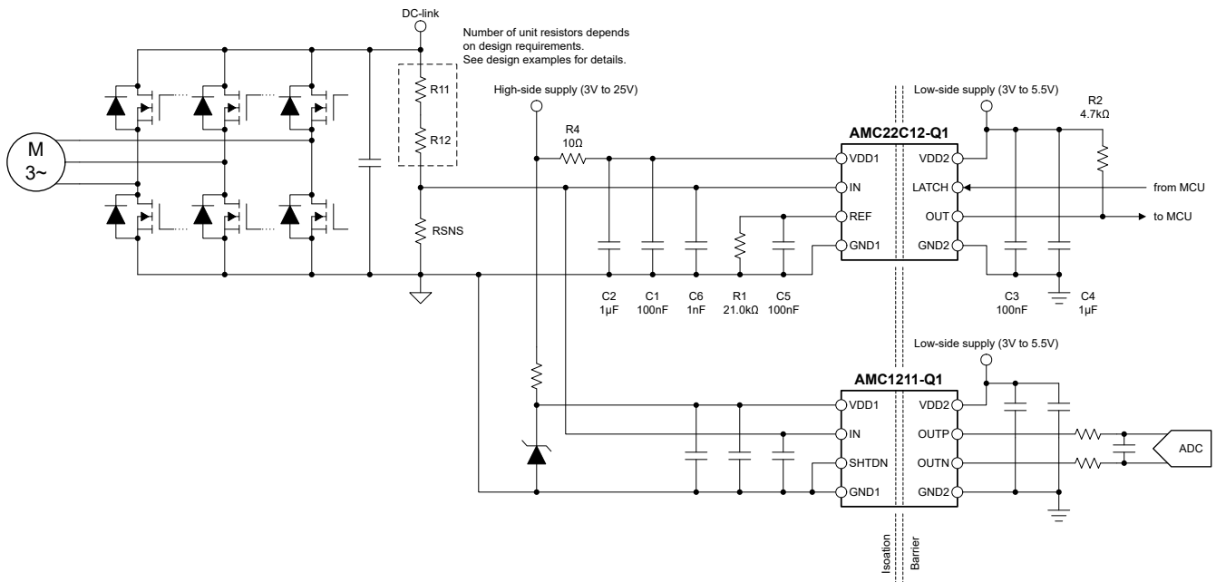
Figure 7-2. Using the AMC22C12-Q1 for Overvoltage Detection
