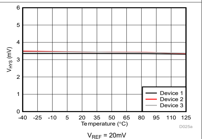
Figure 5-11. Trip Threshold Hysteresis vs Temperature
