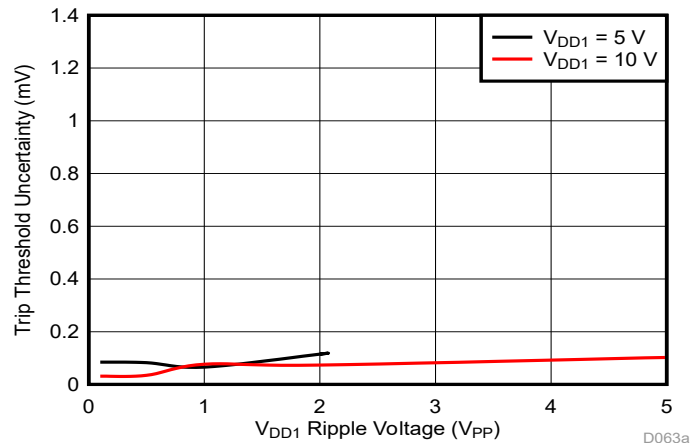
Figure 7-3. Trip Threshold Sensitivity to VDD1 Ripple Voltage ( f_{RIPPLE} = 10\text{kHz} )
