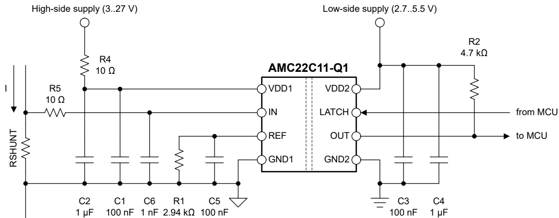
Figure 7-4. Decoupling of the AMC22C11-Q1
