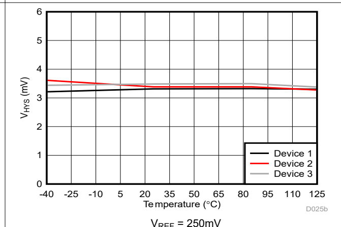
Figure 5-17. Trip Threshold Hysteresis vs Temperature
