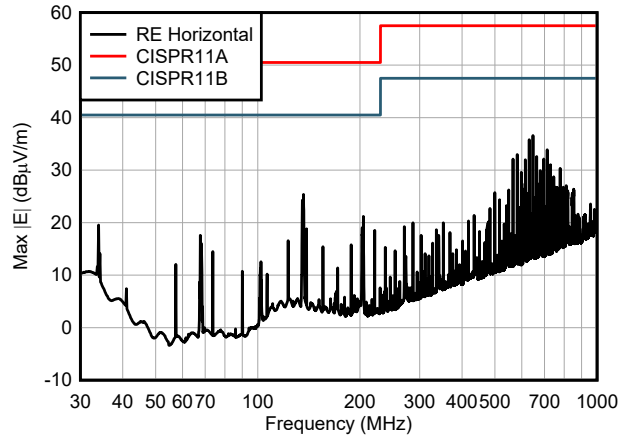
Figure 9-6. AMC131M01 Horizontal Radiated Emission CISPR11 Measurement
