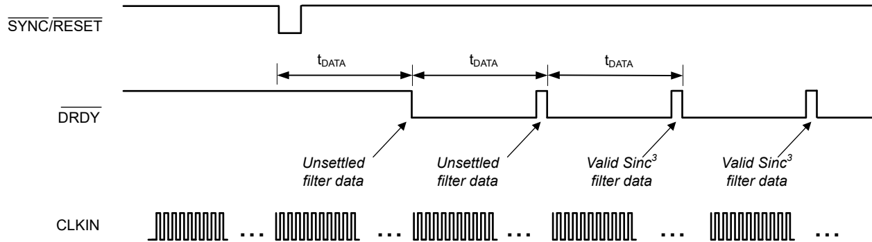
Figure 8-16. Synchronization Timing for \text{OSR} = 1024
