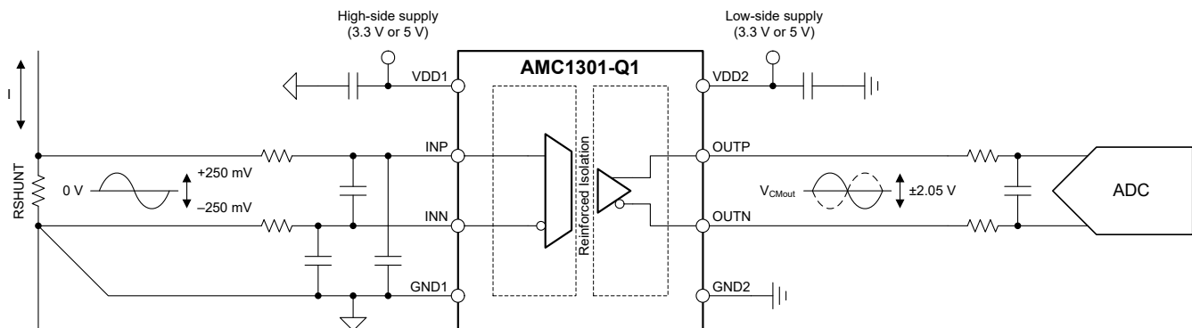
Typical Application
