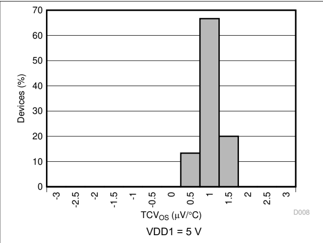
Figure 6-12. Input Offset Drift Histogram
