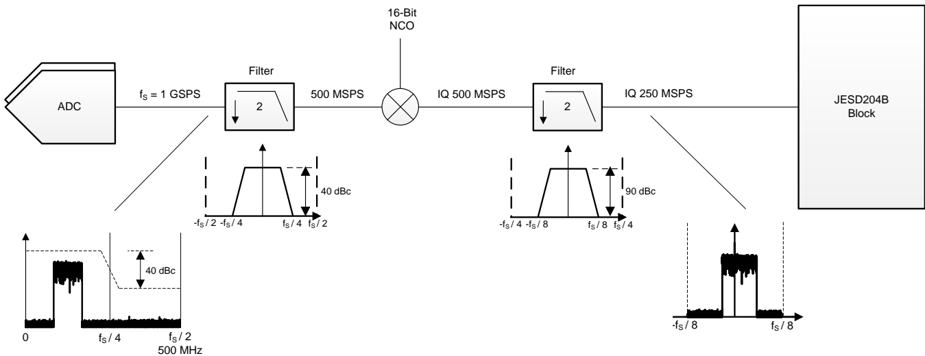
Figure 55. Operating Mode 1
