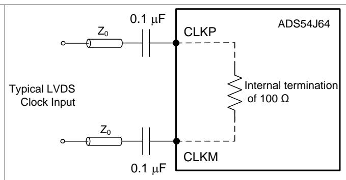
Figure 48. LVDS Clock Driving Circuit
