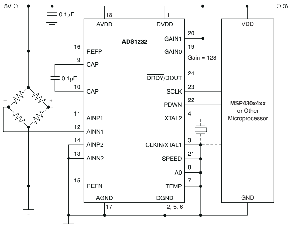
Figure 9-1. Weigh-Scale Application
