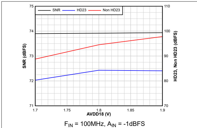
Figure 6-19. AC Performance vs AVDD18
