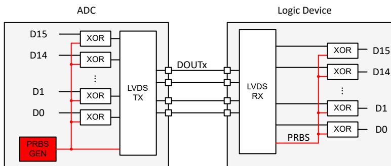
Figure 8-63. Output Scrambler
