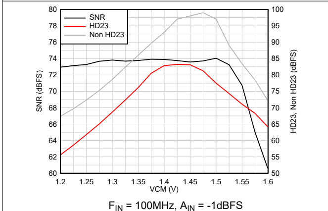
Figure 6-21. AC Performance vs VCM
