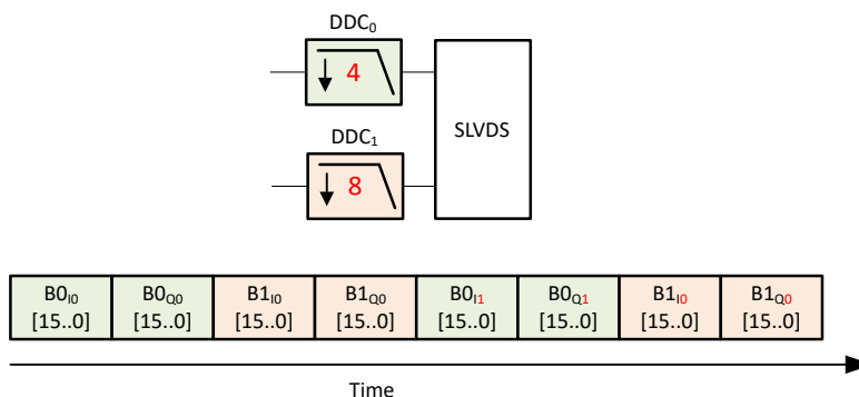
Figure 8-21. Unequal Decimation Factors
