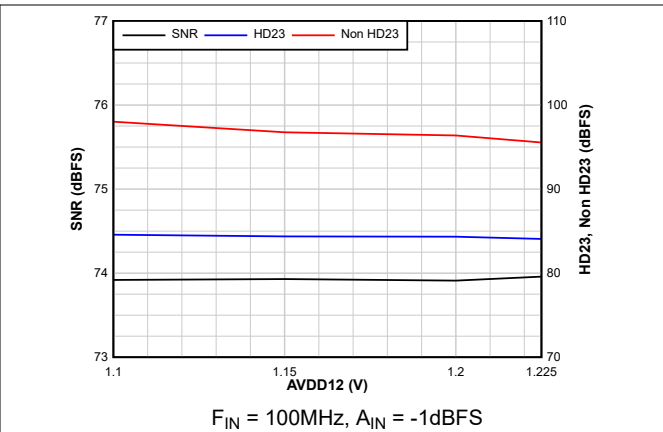
Figure 6-20. AC Performance vs AVDD12
