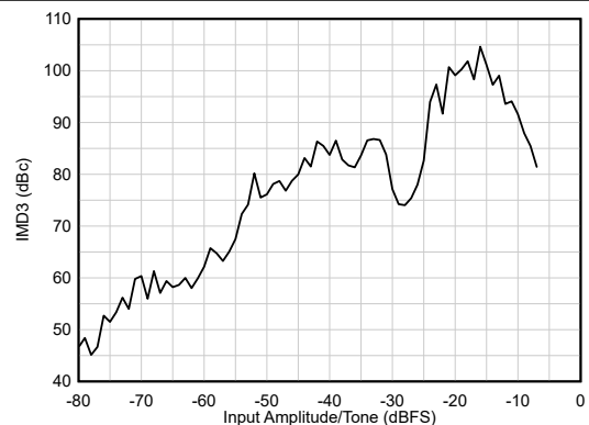
Figure 6-15. AC Performance vs A_{IN}
