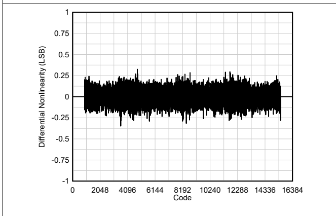
Figure 6-23. DNL
