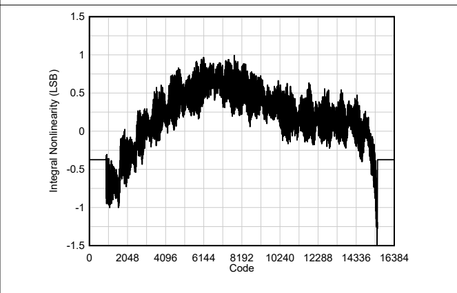
Figure 6-24. INL
