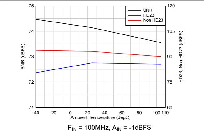
Figure 6-22. AC Performance vs Temperature
