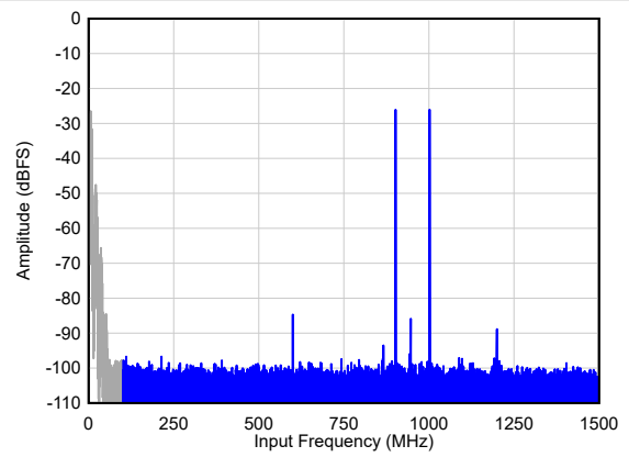
Figure 6-81. Two Tone FFT at F_{IN} = 900/1000 MHz
