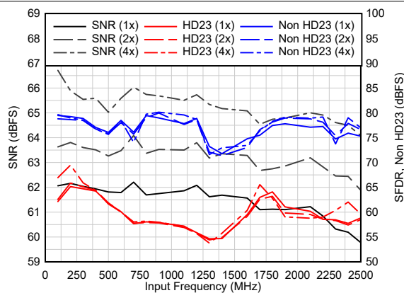
Figure 6-82. AC Performance vs F_{IN}
