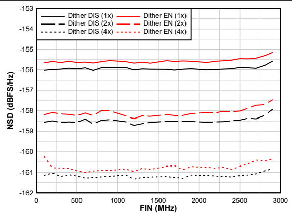
Figure 6-85. NSD Performance vs F_{IN}
