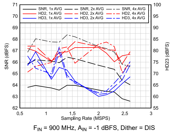
Figure 6-36. AC Performance vs F_S
