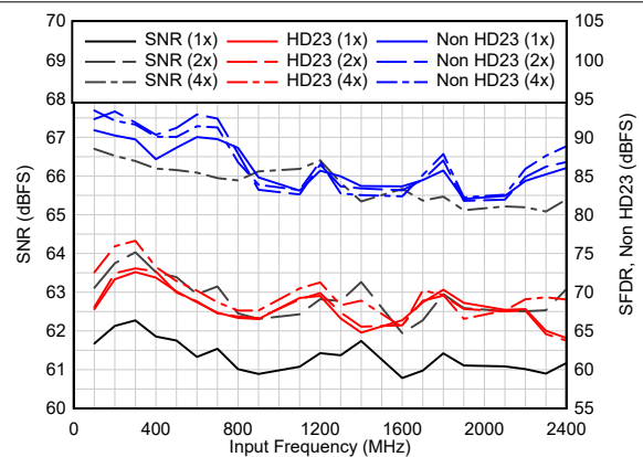
Figure 6-83. AC Performance vs F_{IN}
