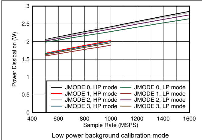
Figure 5-79. Quad Channel, Power Dissipation vs F_S and JMODES 0 - 3
