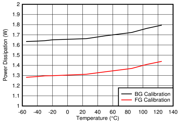
Figure 5-123. Single Channel, Power Dissipation vs Temperature
