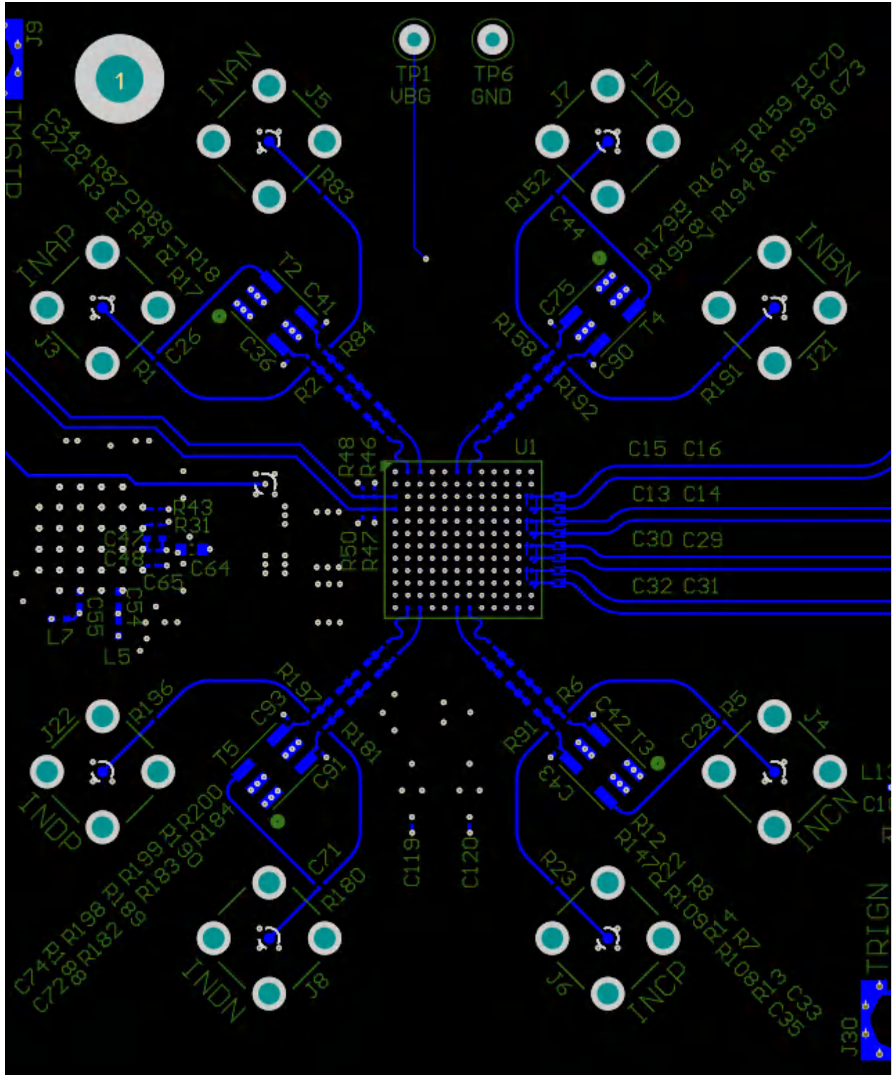
Figure 7-5. Top Layer Routing: Analog Inputs (INA \pm , INB \pm , INC \pm , IND \pm ), TMSTP \pm and D[3:0] \pm Routing
