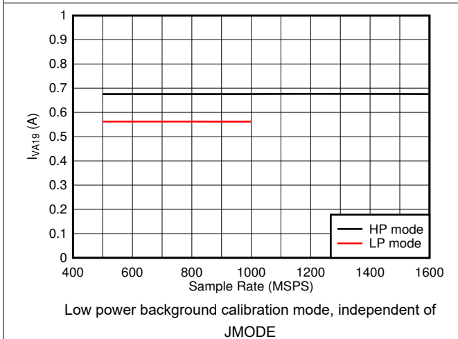
Figure 5-83. Quad Channel, I_{VA19} vs F_S
