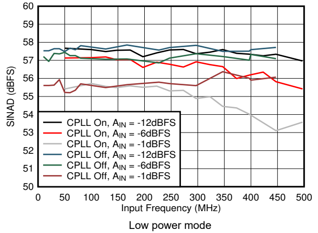
Figure 5-56. SINAD vs A_{IN} and C-PLL
