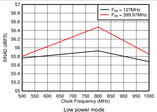
Figure 7-30. SINAD vs Sample Rate
