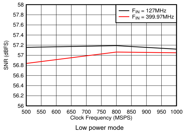
Figure 7-28. SNR vs Sample Rate
