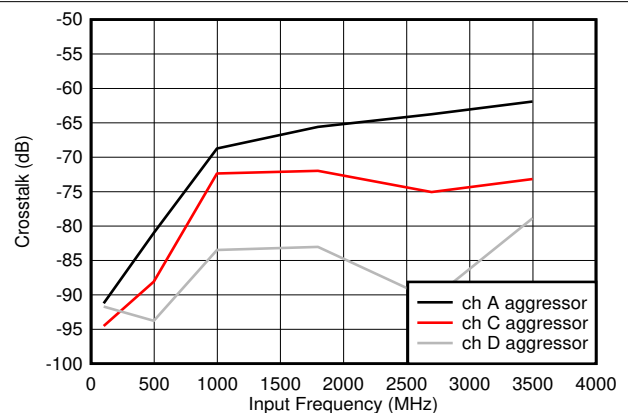
Figure 7-78. Crosstalk to Channel B vs F_{IN}
