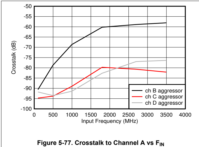
Figure 5-77. Crosstalk to Channel A vs F_{IN}
