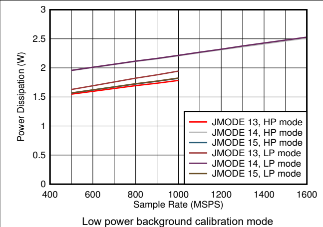
Figure 7-82. Quad Channel, Power Dissipation vs F_S and JMODE 13 - 15
