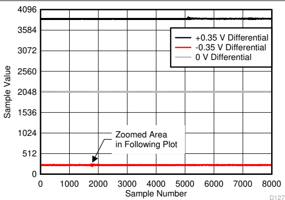
DES_EN = 1, f_s = 6400 \text{ MSPS} , DC input
