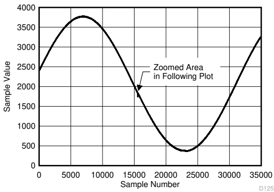
DES_EN = 1, f_s = 6400 \text{ MSPS} , f_{\text{IN}} = 3199.9 \text{ MHz}
