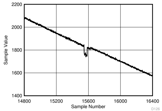
DES_EN = 1, f_s = 6400 \text{ MSPS} , f_{\text{IN}} = 3199.9 \text{ MHz}
