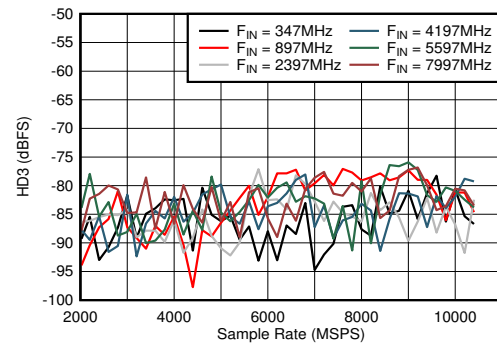
Figure 5-40. DES Mode: HD3 vs Sample Rate and Input Frequency
