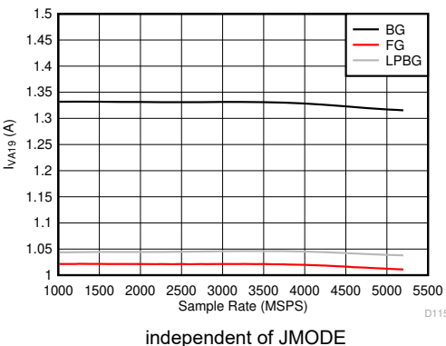
Figure 5-131. Dual Channel Mode: I_{VA19} vs Sample Rate
