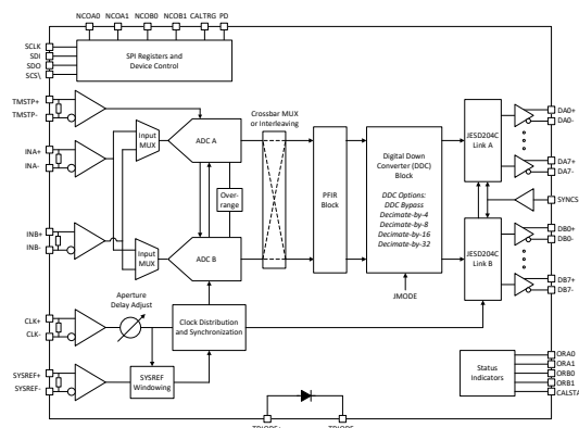
ADC12DJ5200-EP Block Diagram
