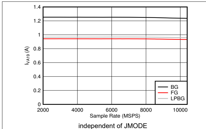
Figure 5-123. DES Mode: I_{VA19} vs Sample Rate
