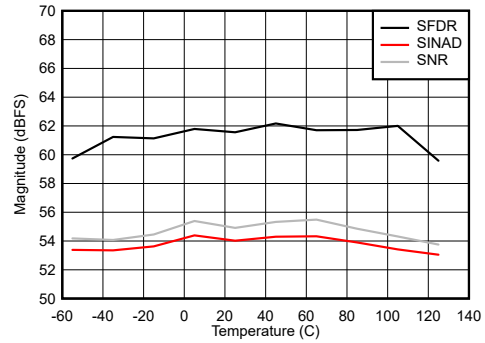
FG calibration at each temperature Figure 6-92. DES Mode: SNR, SINAD and SFDR vs Temperature
