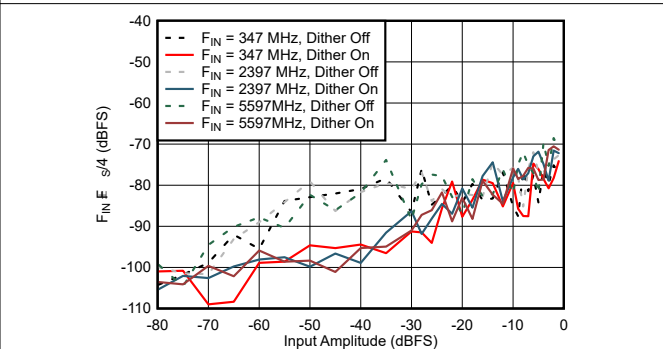
Figure 6-66. DES Mode: F_{\text{IN}} \pm F_{\text{IN}}/4 vs Input Amplitude and Dither
