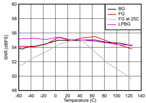
FG25 is calibrated at 25°C and held at other temperatures, other modes recalibrated at each temperature Figure 6-96. DES Mode: SNR vs Temperature and Calibration Mode
