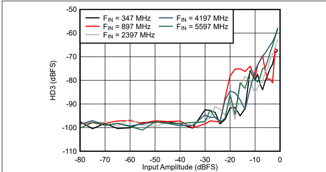
Figure 6-61. DES Mode: HD3 vs Input Amplitude and Frequency
