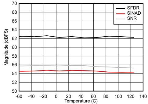
FG calibration at each temperature Figure 6-94. Dual Channel Mode: SNR, SINAD and SFDR vs Temperature
