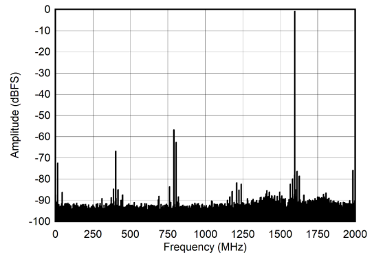
Figure 6-22. Dual Channel Mode: Single Tone FFT at 5597 MHz
