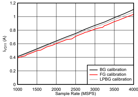
JMODE = 1 Figure 6-118. DES Mode: I_{VD11} vs Sample Rate
