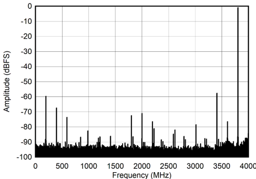
Figure 6-11. DES Mode: Single Tone FFT at 4197 MHz
