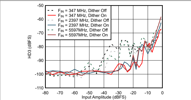
Figure 6-62. DES Mode: HD3 vs Input Amplitude and Dither
