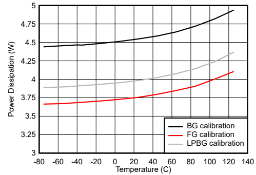
Figure 6-137. Dual Channel Mode: Power Dissipation vs Temperature
