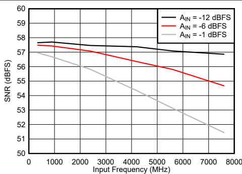
Figure 6-77. DES Mode: SNR vs Input Frequency
