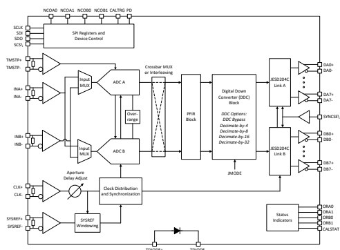
ADC12DJ4000RF Block Diagram
