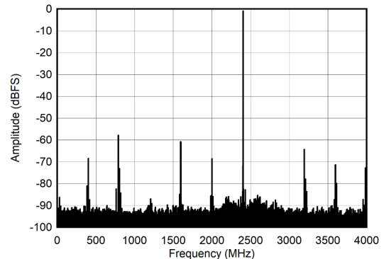
Figure 6-12. DES Mode: Single Tone FFT at 5597 MHz
