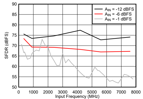
Figure 6-84. Dual Channel Mode: SFDR vs Input Frequency
