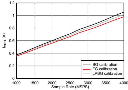
JMODE = 30 Figure 6-120. DES Mode: I_{VD11} vs Sample Rate
