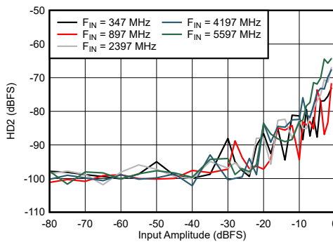
Figure 6-59. DES Mode: HD2 vs Input Amplitude and Frequency
