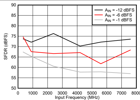
Figure 6-78. DES Mode: SFDR vs Input Frequency
