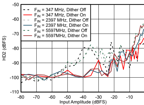
Figure 6-60. DES Mode: HD2 vs Input Amplitude and Dither
