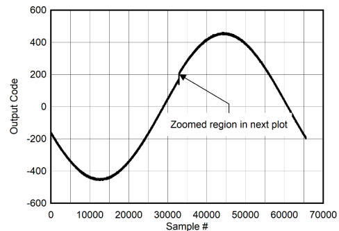
Figure 6-139. Background Calibration Core Transition (AC Signal)
