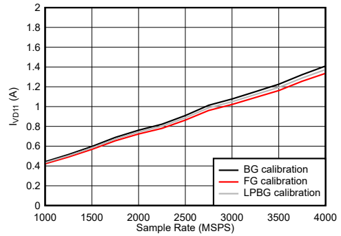
JMODE = 61 Figure 6-121. DES Mode: I_{VD11} vs Sample Rate
