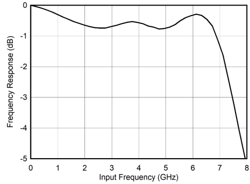
Relative to 0Hz, FG calibration Figure 6-2. DES Mode: Input Response vs Input Frequency
