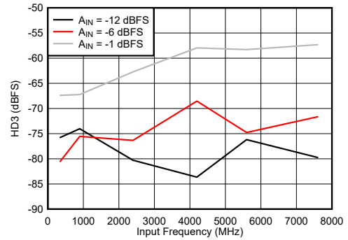
Figure 6-80. DES Mode: HD3 vs Input Frequency
