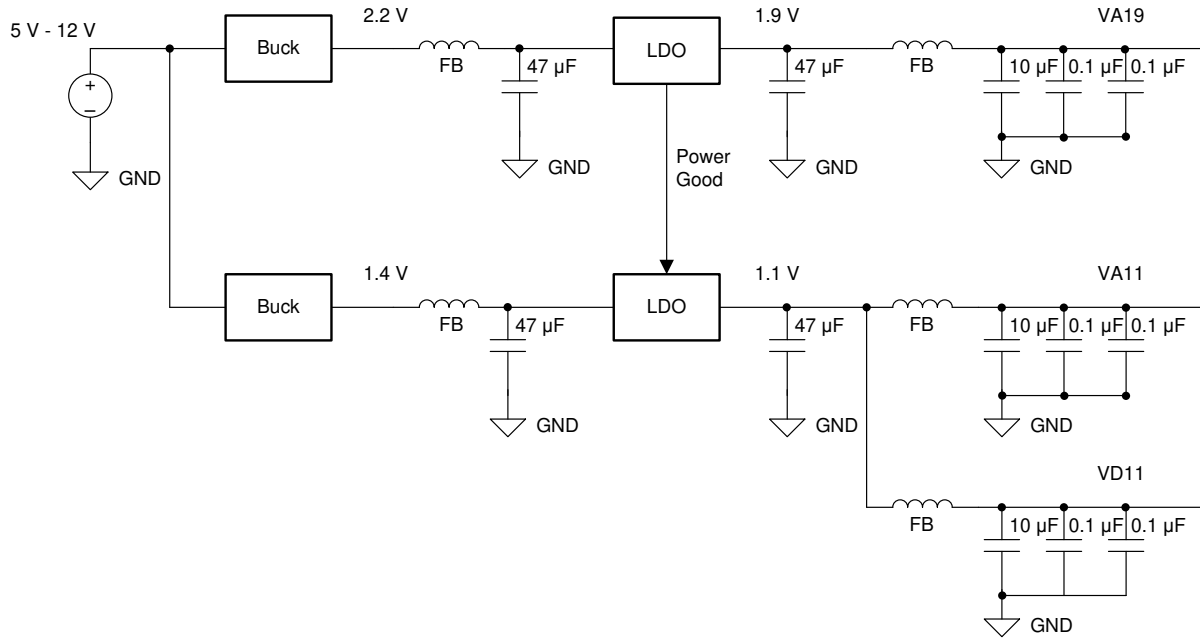
Figure 8-4. LDO Linear Regulator Approach Example
