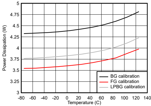
Figure 6-136. DES Mode: Power Dissipation vs Temperature
