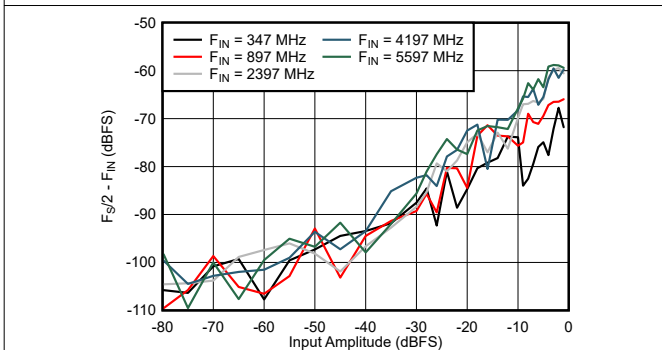
Figure 6-63. DES Mode: F_s/2 - F_{\text{IN}} vs Input Amplitude and Frequency
