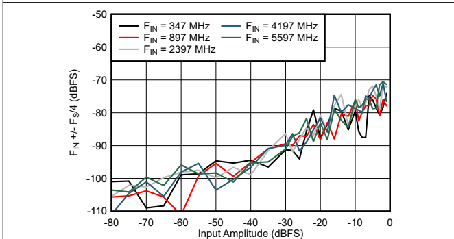
Figure 6-65. DES Mode: F_{\text{IN}} \pm F_{\text{IN}}/4 vs Input Amplitude and Frequency
