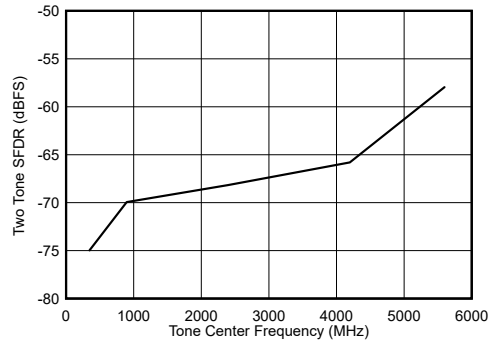
Figure 6-110. DES Mode: Two Tone SFDR vs Input Frequency
