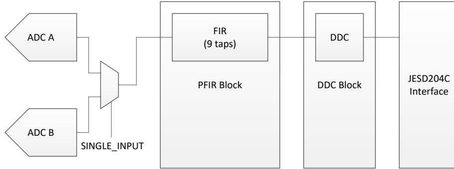
Figure 7-5. Single Channel Equalization PFIR Block Diagram
