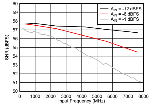
Figure 6-82. DES Mode: F_{\text{IN}} \pm F_s/4 vs Input Frequency
