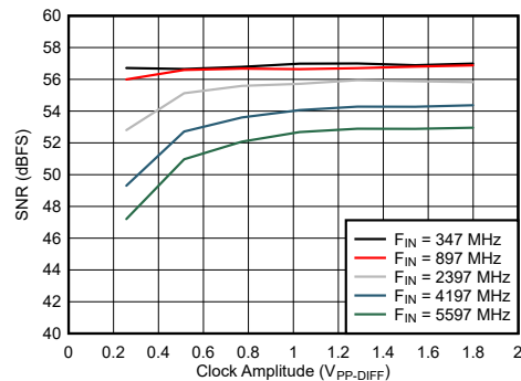
Figure 6-90. Dual Channel Mode: SNR vs Clock Amplitude
