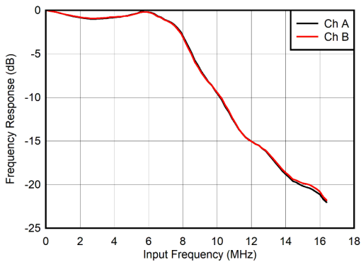
Relative to 0Hz, FG calibration Figure 6-3. Dual Channel Mode: Input Amplitude vs Input Frequency
