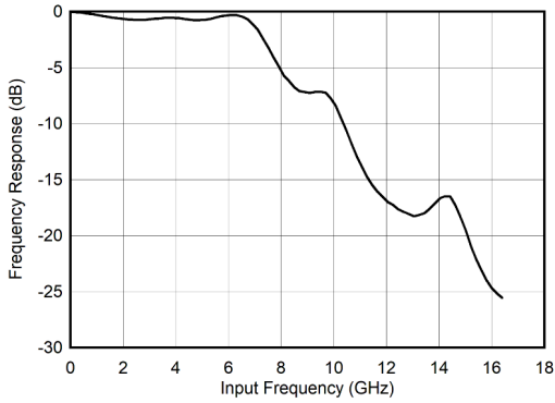
Relative to 0Hz, FG calibration Figure 6-1. DES Mode: Input Amplitude vs Input Frequency
