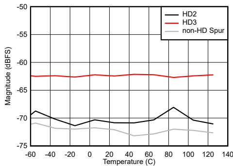
FG calibration at each temperature Figure 6-93. DES Mode: HD2, HD3 and Worst non-HD Spur vs Temperature
