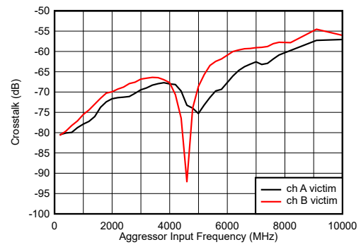
Dual channel mode, JMODE 3 Figure 6-5. Crosstalk vs Input Frequency
