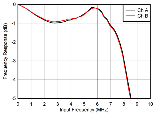
Relative to 0Hz, FG calibration Figure 6-4. Input Response vs Input Frequency (zoomed)
