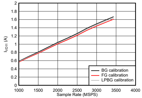
JMODE = 21 Figure 6-119. DES Mode: I_{VD11} vs Sample Rate
