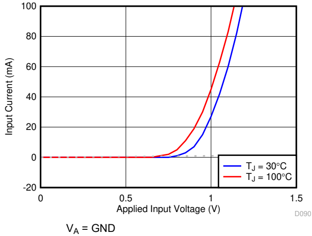
Figure 8-7. ESD Diode Current
