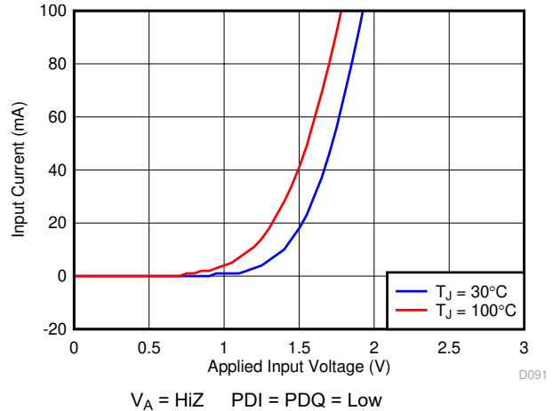
Figure 8-8. ESD Diode Current
