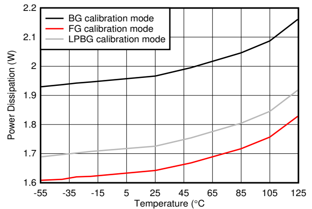
Figure 7-124. Dual Channel, Power Dissipation vs Temperature
