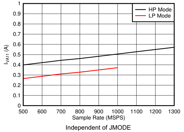
Figure 7-86. Quad Channel, I_{VA11} vs FS
