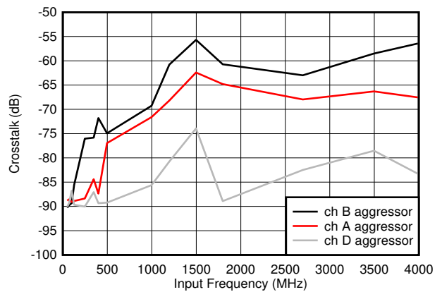
Figure 7-60. Crosstalk to Channel B vs F_{IN}
