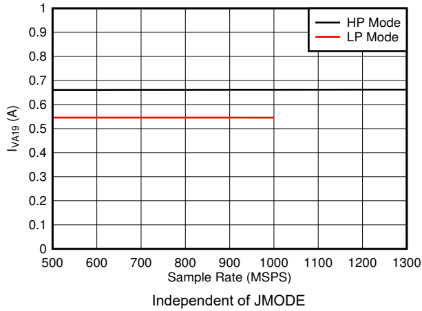
Figure 7-85. Quad Channel, I_{VA19} vs FS
