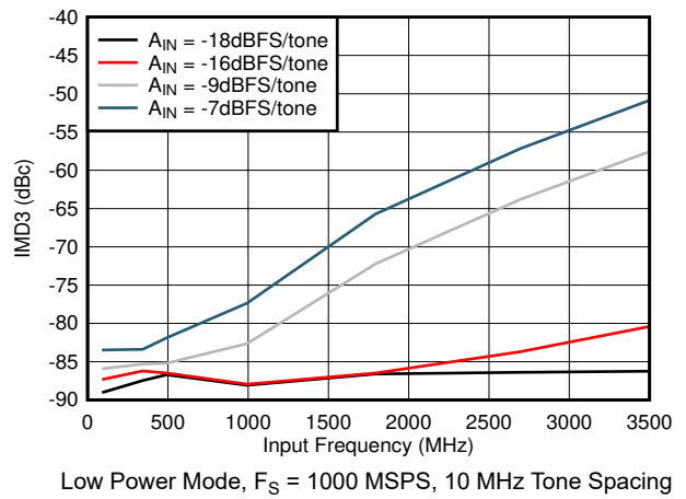
Figure 7-58. IMD3 vs Input Frequency
