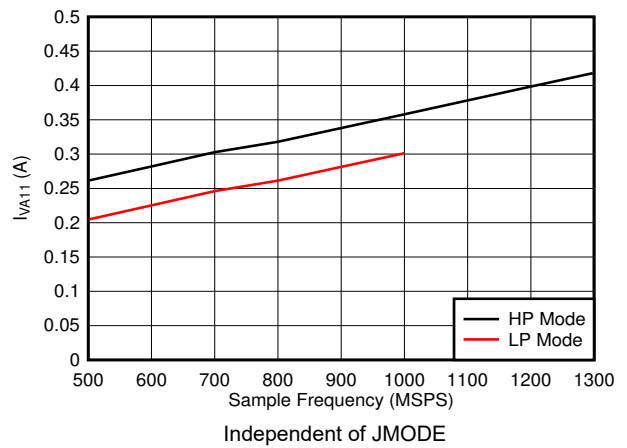
Figure 7-106. Single Channel, I_{VA11} vs FS
