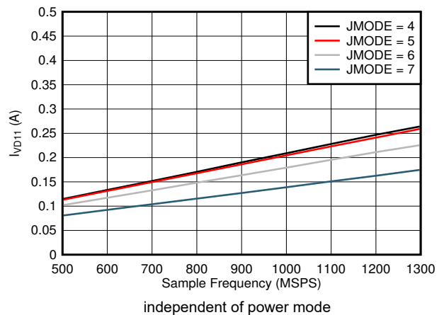
Figure 7-108. Single Channel, I_{VD11} vs FS and JMODE 4 - 7
