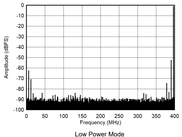
Figure 5-12. Single Tone FFT at 1197MHz and -1dBFS
