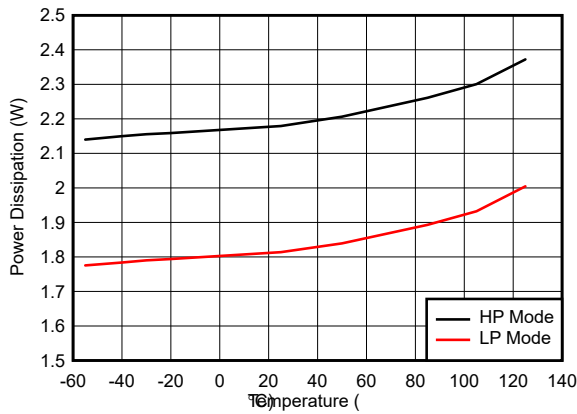
Figure 5-113. Quad Channel, Power Dissipation vs Temperature
