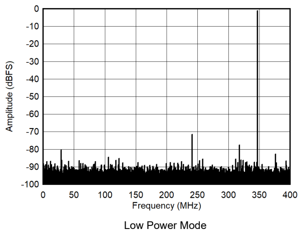
Figure 5-11. Single Tone FFT at 347MHz and -1dBFS
