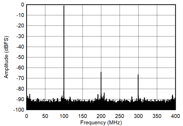
Figure 5-10. Single Tone FFT at 100MHz and -1dBFS
