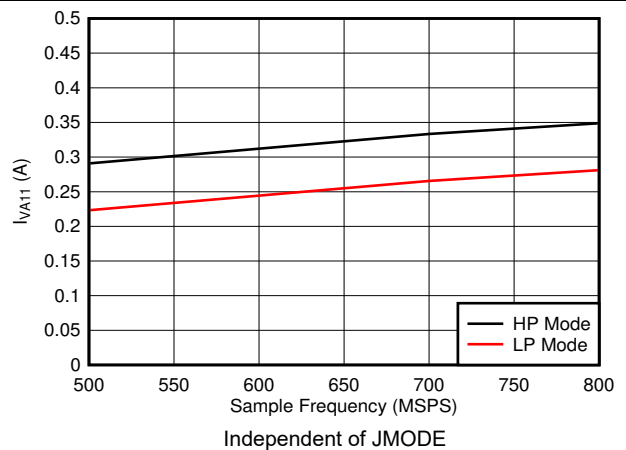
Figure 5-86. Dual Channel, I_{VA11} vs F_S
