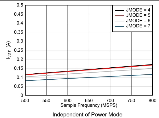
Figure 5-98. Single Channel, I_{VD11} vs F_S for JMODES 4 - 7
