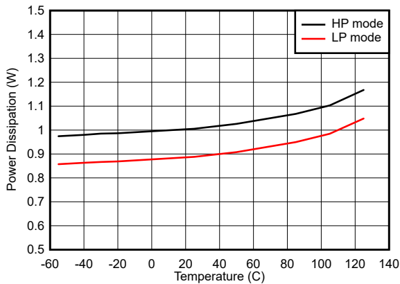
Figure 5-113. Quad Channel, Power Dissipation vs Temperature
