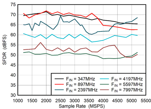
Figure 6-47. Dual Channel Mode: SFDR vs Sample Rate
