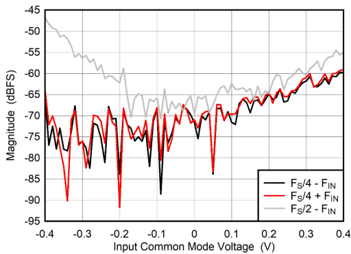
Figure 6-99. DES Mode: F_S/2 - F_{IN} , F_S/4 \pm F_{IN} vs Input Common Mode Voltage
