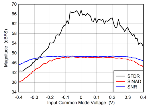
Figure 6-98. DES Mode: SNR, SFDR and SINAD vs Input Common Mode Voltage
