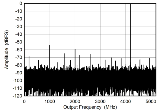
Figure 6-8. DES Mode: Single Tone FFT at 4197 MHz
