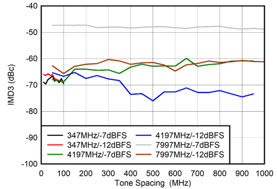
Figure 6-102. DES Mode: IMD3 vs Tone Spacing
