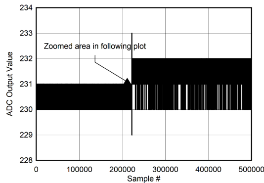
Figure 6-121. Background Calibration Core Transition (DC Signal)
