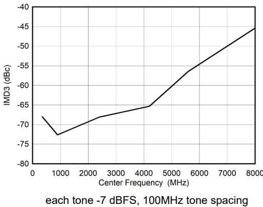
Figure 6-105. Dual Channel Mode: IMD3 vs Input Frequency
