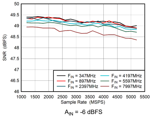
Figure 6-45. Dual Channel Mode: SNR vs Sample Rate
