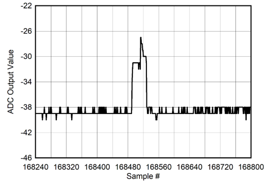
Figure 6-120. Background Calibration Core Transition (AC Signal Zoomed)
