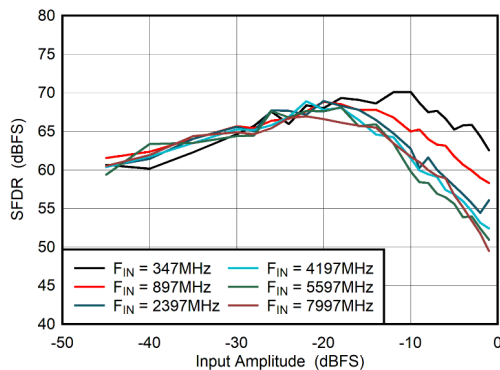
Figure 6-59. DES Mode: SFDR vs Input Amplitude
