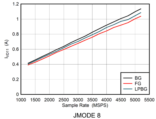
Figure 6-116. Dual Channel Mode: I_{V_{D11}} vs Sample Rate
