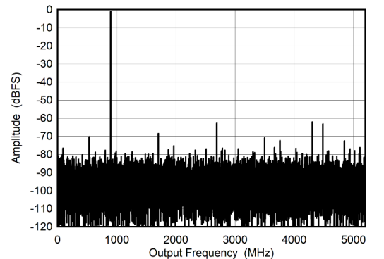
Figure 6-6. DES Mode: Single Tone FFT at 897 MHz
