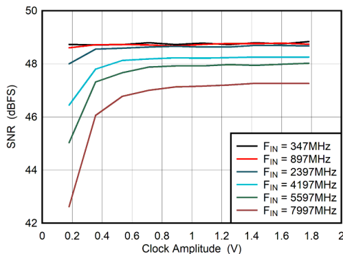
Figure 6-83. Dual Channel Mode: SNR vs Clock Amplitude
