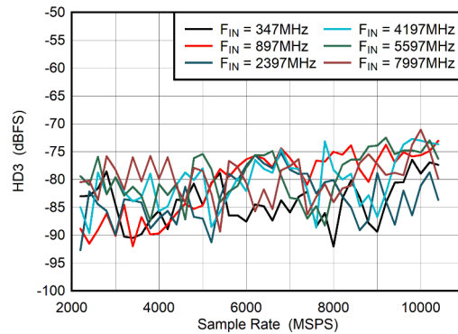
Figure 6-40. DES Mode: HD3 vs Sample Rate
