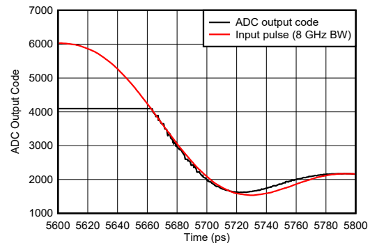
Figure 6-124. Pulse Overdrive Recovery Zoomed
