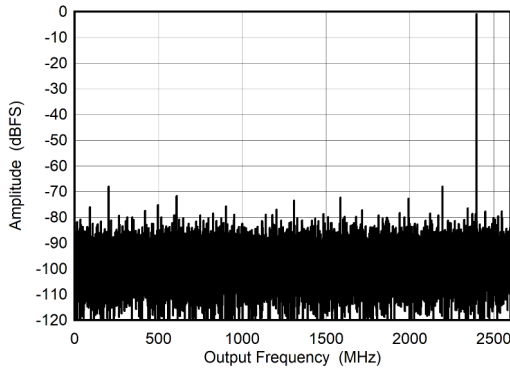
Figure 6-19. Dual Channel Mode: Single Tone FFT at 2397 MHz
