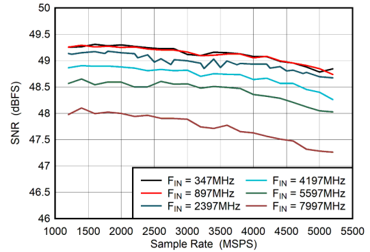
Figure 6-44. Dual Channel Mode: SNR vs Sample Rate
