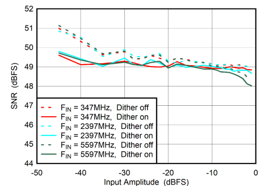
Figure 6-72. Dual Channel Mode: SNR vs Input Amplitude and Dither
