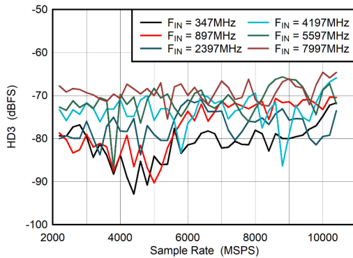
Figure 6-39. DES Mode: HD3 vs Sample Rate
