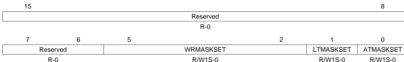
Figure 1-43. Interrupt Mask Set Register (EIMSR)
