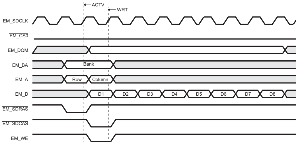
Figure 1-6. Timing Waveform for Basic SDRAM Write Operation
