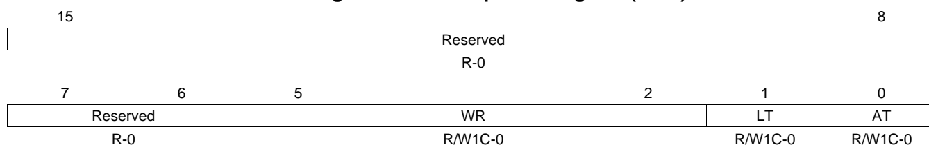
Figure 1-41. Interrupt Raw Register (EIRR)
