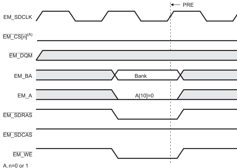
Figure 1-3. Timing Waveform for SDRAM PRE Command
