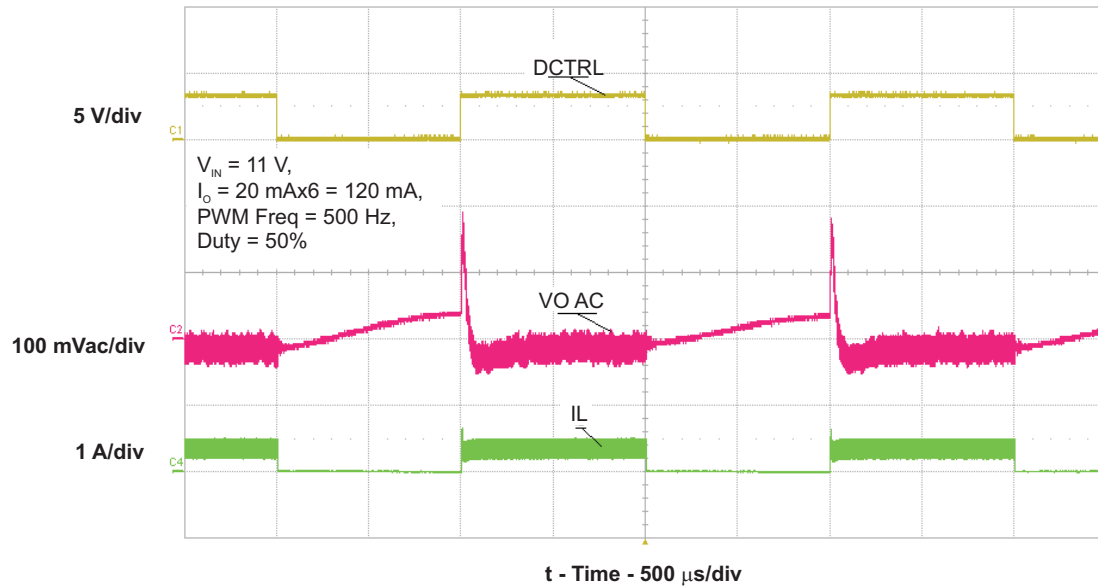
Figure 5. Output Ripple at PWM Dimming with C_o = 4.7\ \mu\text{F}
