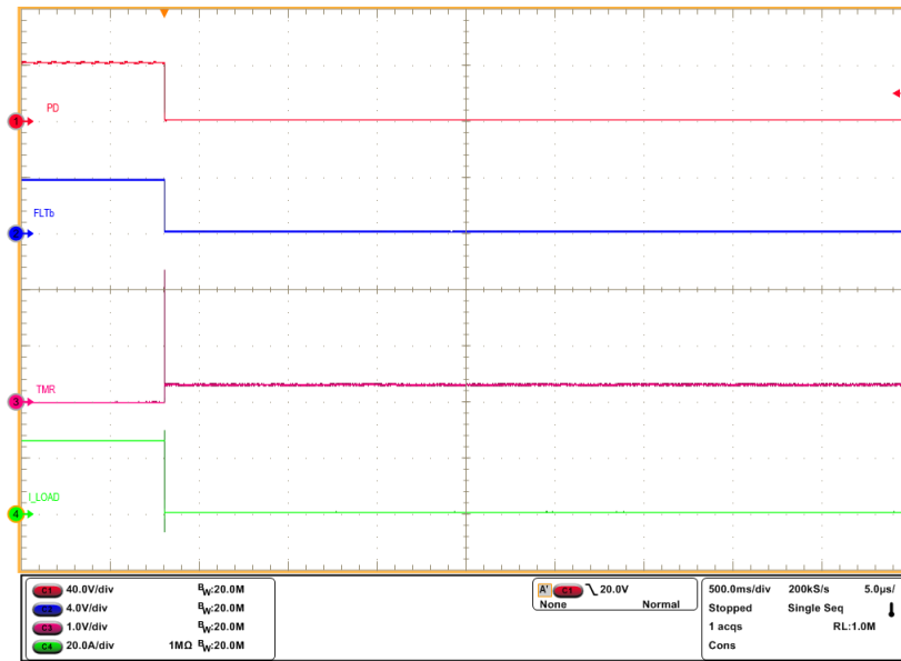
Figure 3-6. Latch-off Response of TPS4810-Q1 for an Overcurrent Fault
