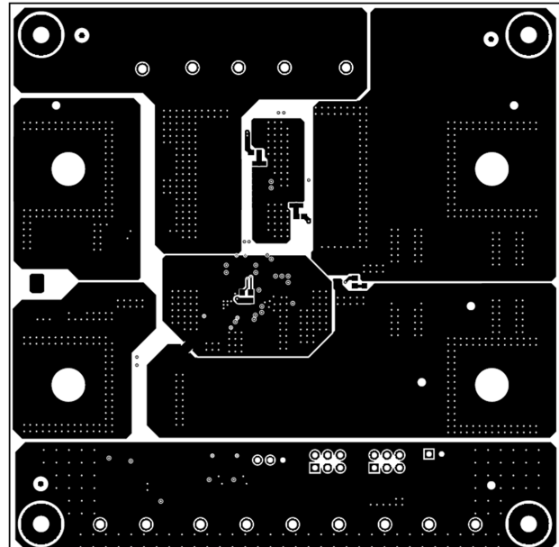
Figure 4-5. TPS4810Q1EVM Board Bottom Layer
