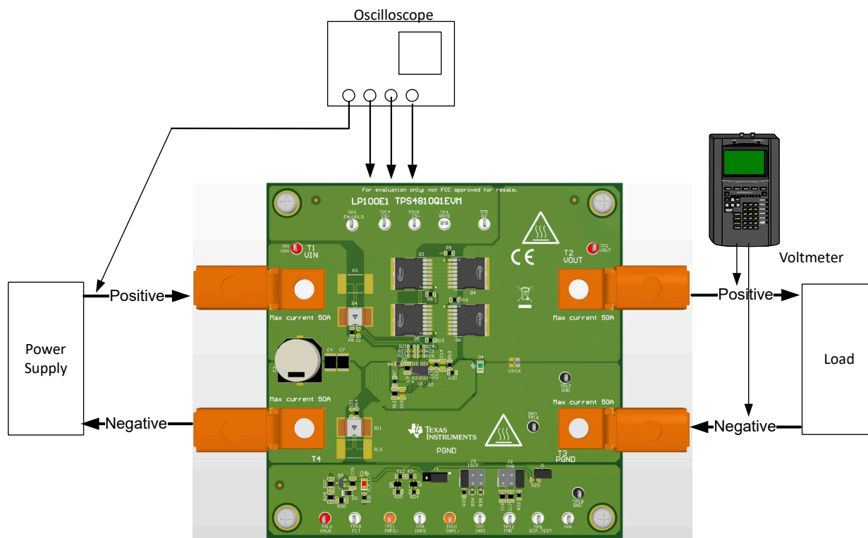
Figure 3-1. TPS4810Q1EVM Setup with Test Equipment
