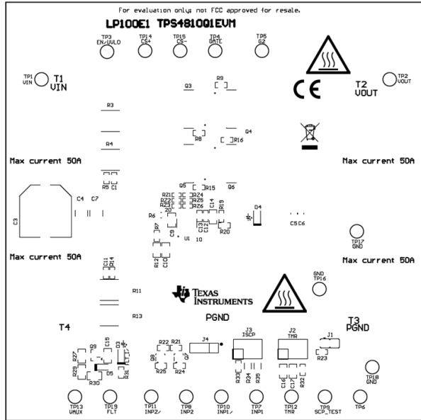
Figure 4-2. TPS4810Q1EVM Board Top Overlay
