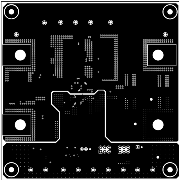
Figure 4-6. TPS4810Q1EVM Board Inner Signal Layer
