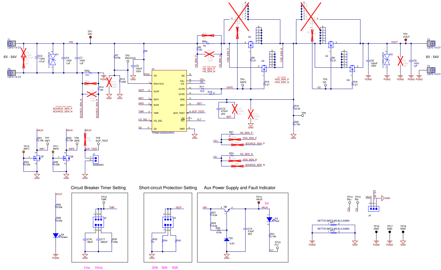
Figure 4-1. TPS4810Q1EVM: Evaluation Module Schematic
