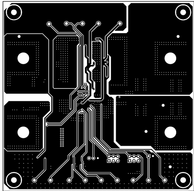
Figure 4-7. TPS4810Q1EVM Board Inner Routing Layer
