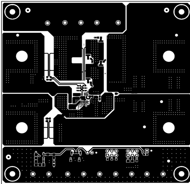
Figure 4-4. TPS4810Q1EVM Board Top Layer
