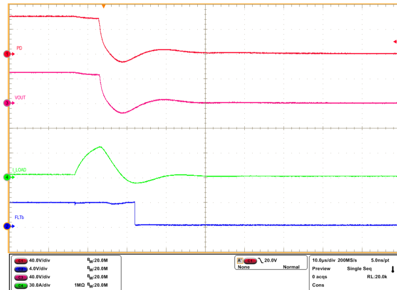
Figure 3-7. Output Short-Circuit Response of TPS4810-Q1
