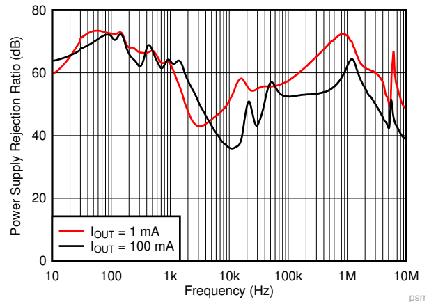
V_{OUT} = 3.3\ \text{V} , C_{IN} = 0\ \mu\text{F} , C_{OUT} = 10\ \mu\text{F}
