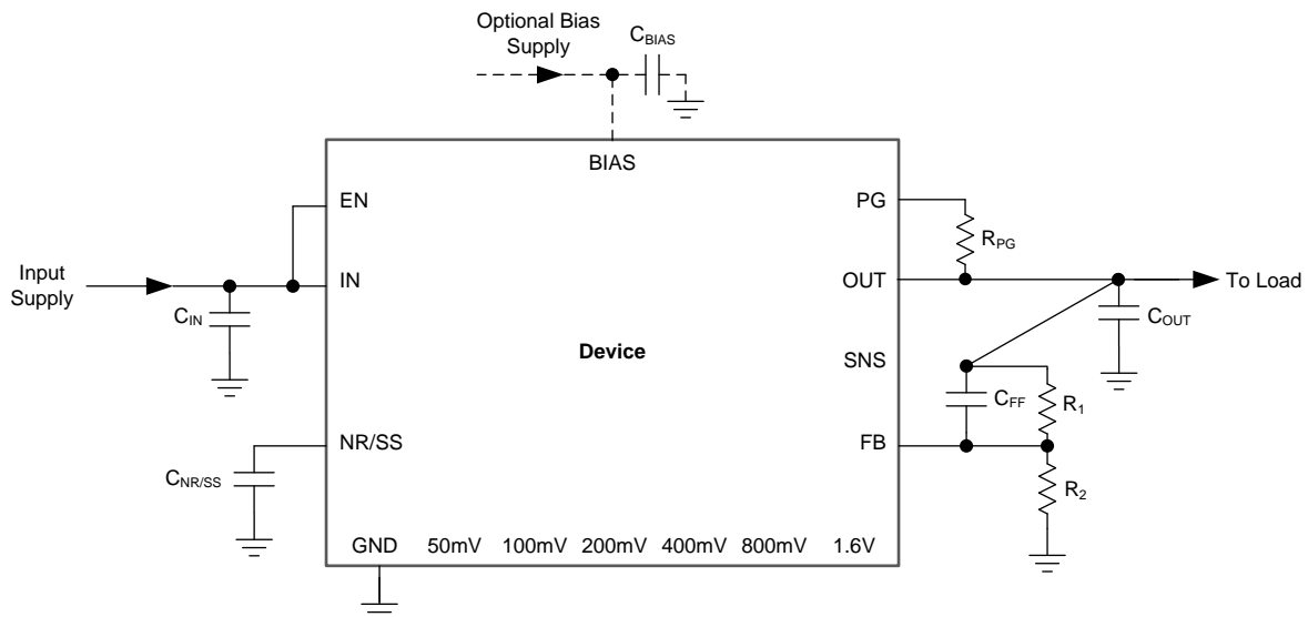
Figure 68. Typical Application
