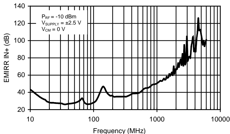
Figure 1. OPA350 EMIRR IN+ vs Frequency
