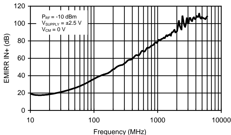
Figure 1. OPA277 EMIRR IN+ vs Frequency
