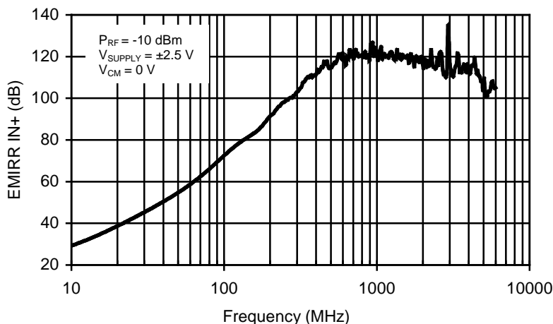
Figure 1. OPA333 EMIRR IN+ vs Frequency
