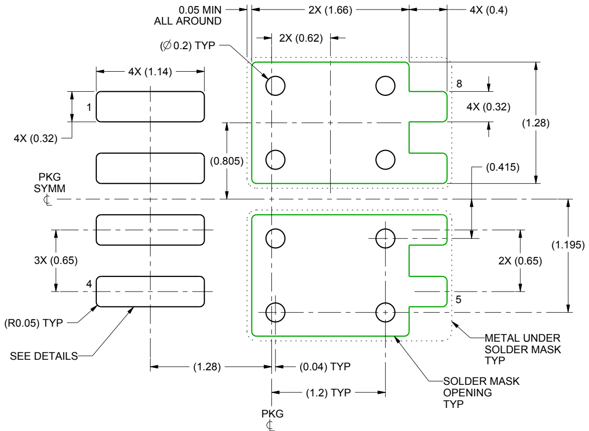
LAND PATTERN EXAMPLE SCALE:25X
