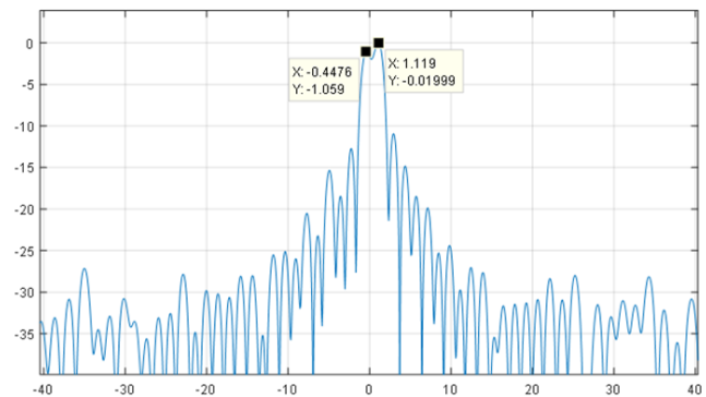
図 22. Range-Doppler FFT Plots Showing Detected, Separated Peaks From Both Reflectors
