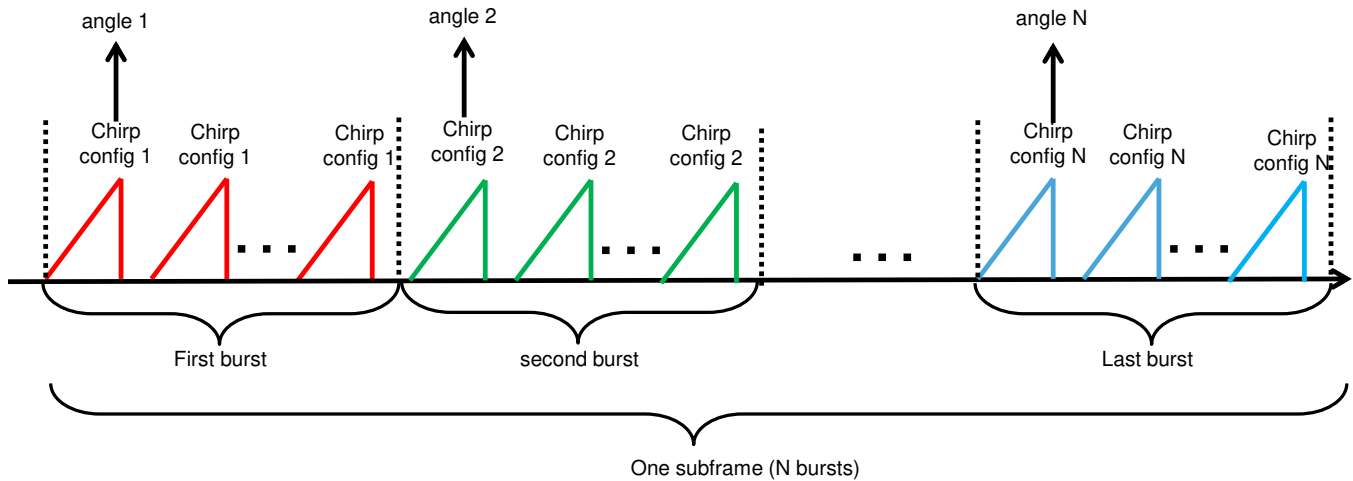
図 11. Frame Based Beam Steering
