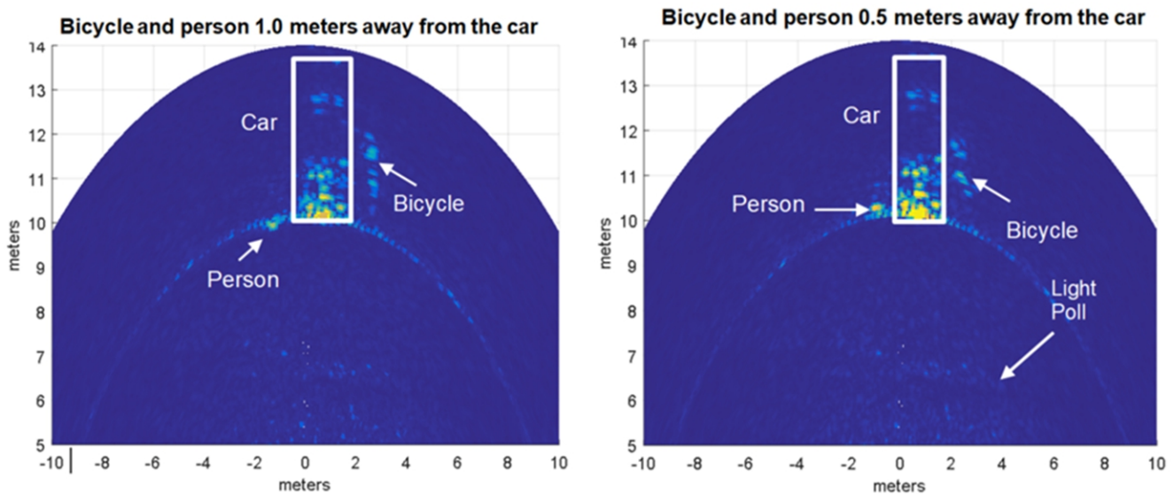
図 26. Bicycle and Person 1.0 Meter (left) and 0.5 Meter (right) Away From Vehicle
