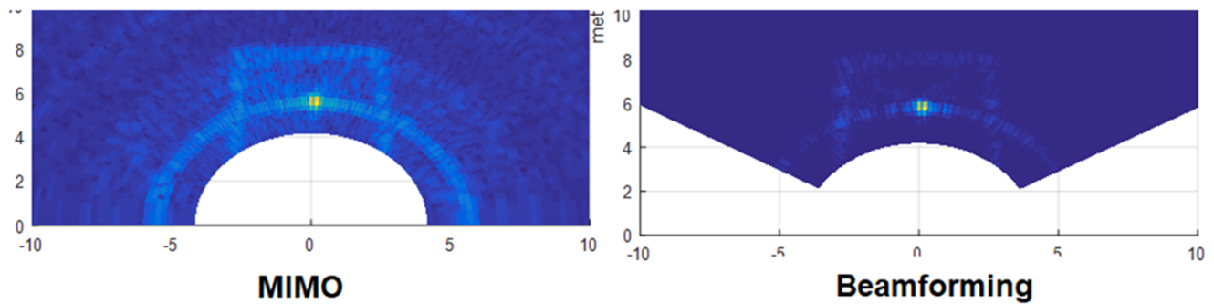
図 18. Heat Map – MIMO and Stitched TX Beamforming – Top Down View
