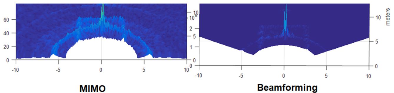
図 19. Heat Map – MIMO and Stitched TX Beamforming – 3D View
