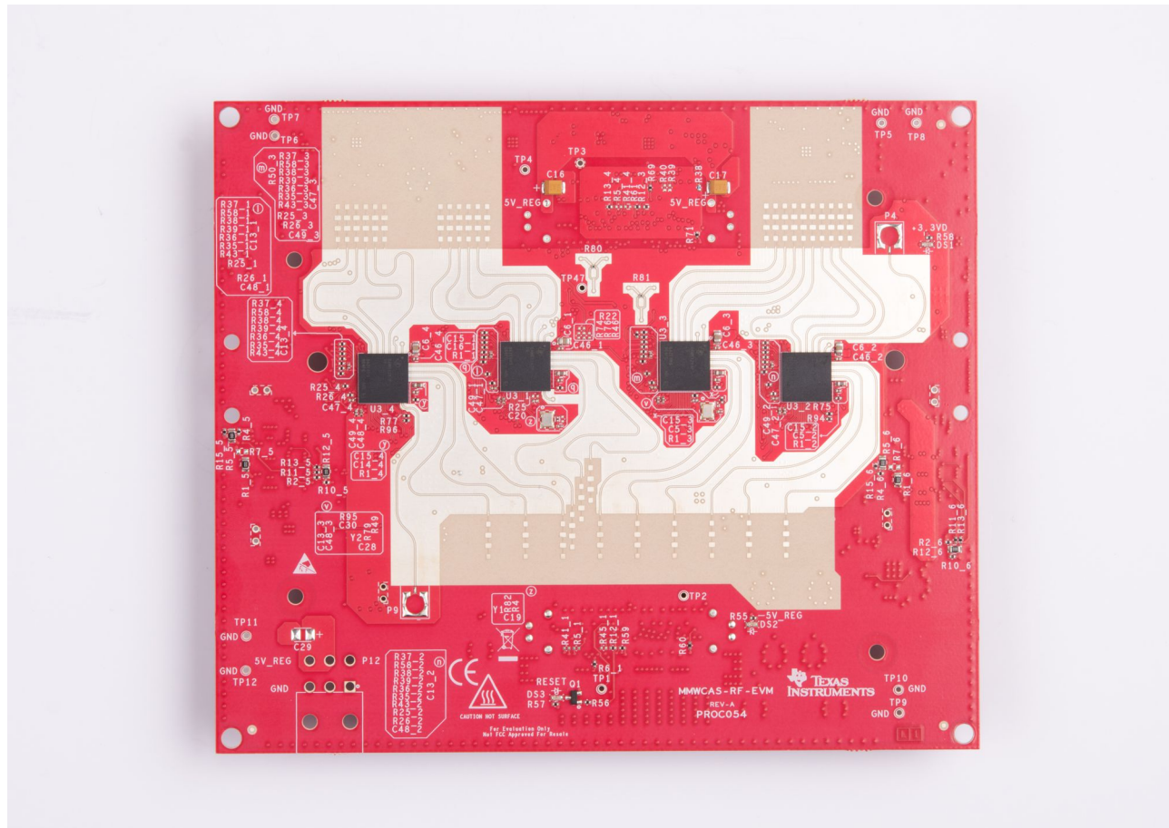
図 1. AWR2243 Four-Device Cascade Radar RF Radar Board
