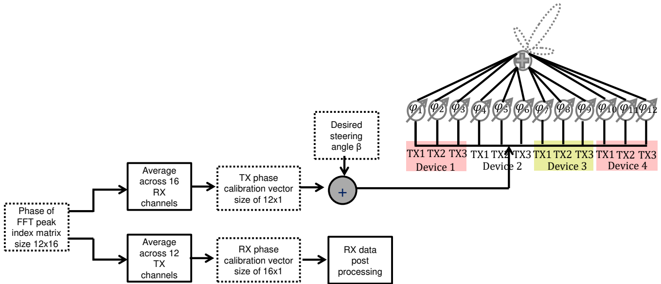
図 15. Calibration in TX Beamforming
