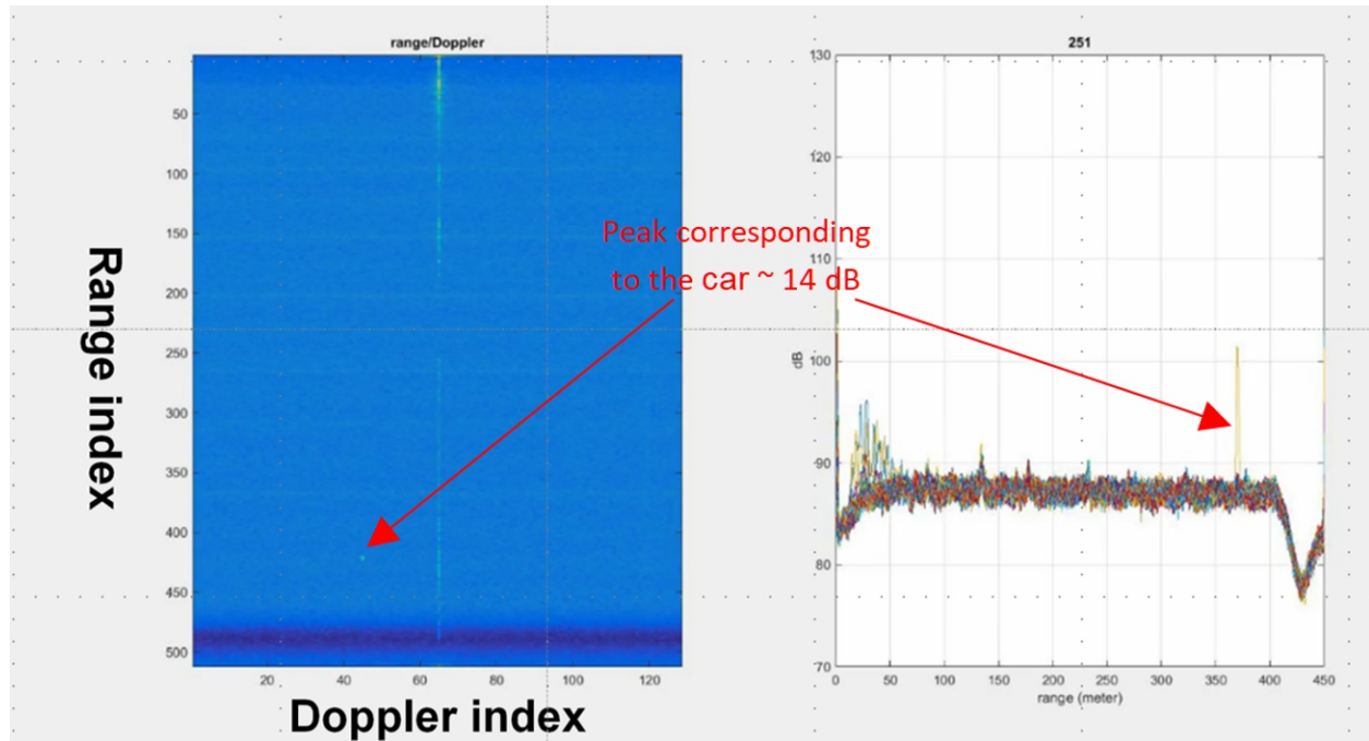
図 31. Range Profile (left), and Doppler-Range Plot of a Vehicle 350 Meters Range
