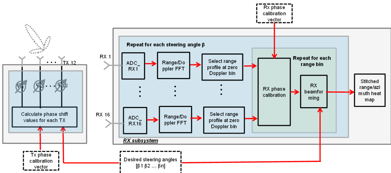
Figure 17. TX Beamforming Signal Processing Chain
