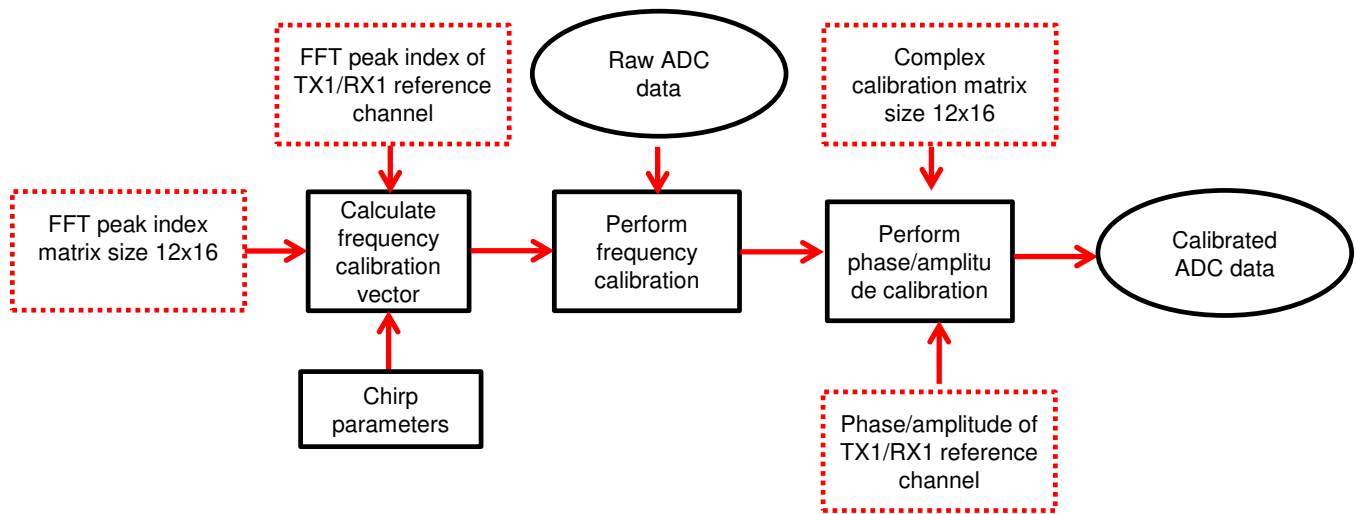
図 14. Flow to Apply Calibration Matrix to ADC Data
