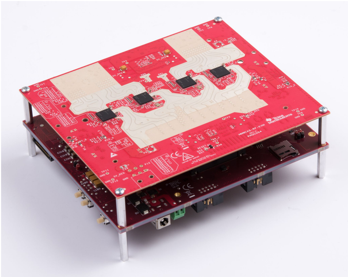
図 20. Four-Device Cascade Radar RF Board with TDA2 Based Capture Board
