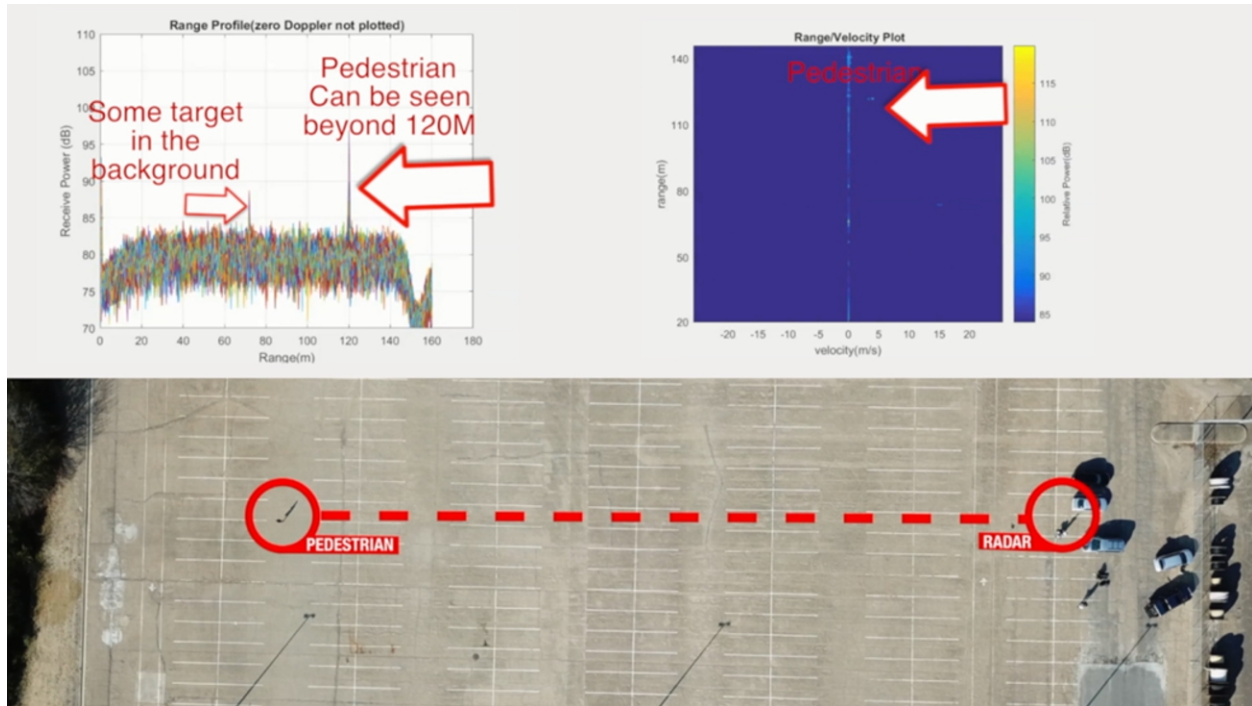
図 30. Range Profile (top left), and Doppler-Range Plot of a Pedestrian Jogging Away From Radar at 120 Meters Range
