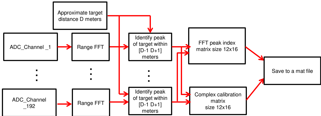
図 13. Flow to Generate Phase and Gain Calibration Matrix
