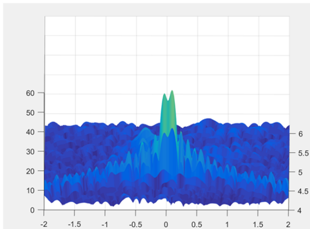
図 22. Range-Doppler FFT Plots Showing Detected, Separated Peaks From Both Reflectors
