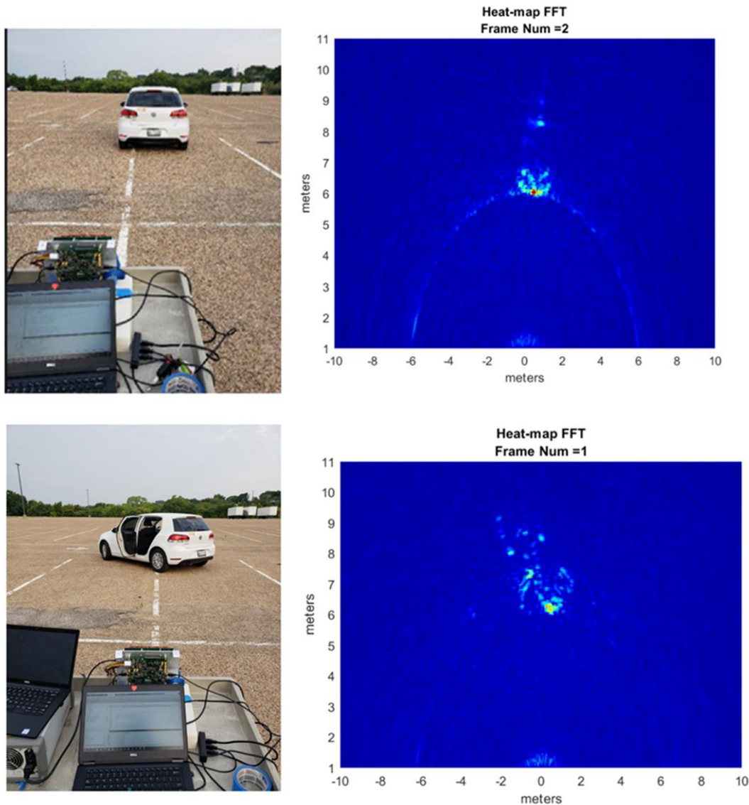
図 27. Car at 0 Degrees (Top) Car with Open Door (Bottom) Orientation and Corresponding Azimuth Range Heatmapp
