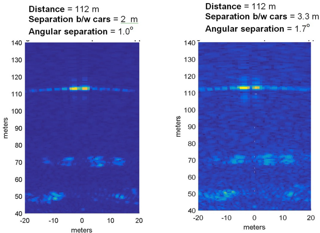
図 24. Two-Car Angular Separation Test Results
