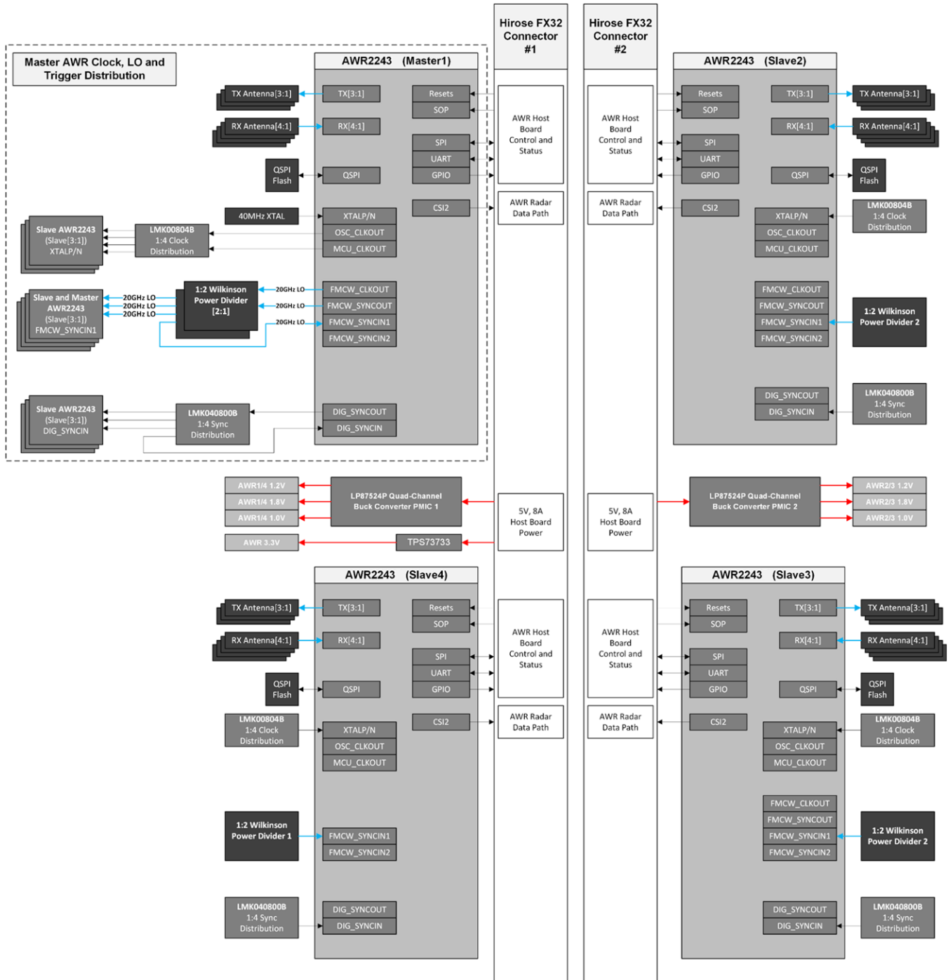
Figure 2. Cascade Radar RF Board System Block Diagram
