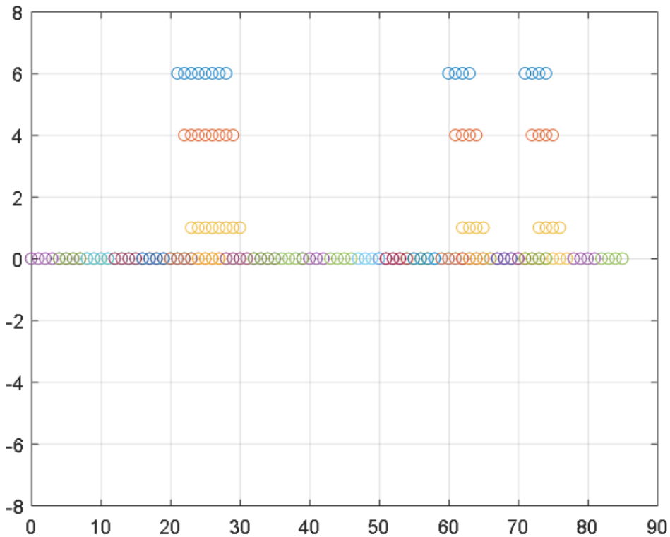
図 7. 4-Device Cascade Virtual MIMO Array with 12 TX and 16 RX
