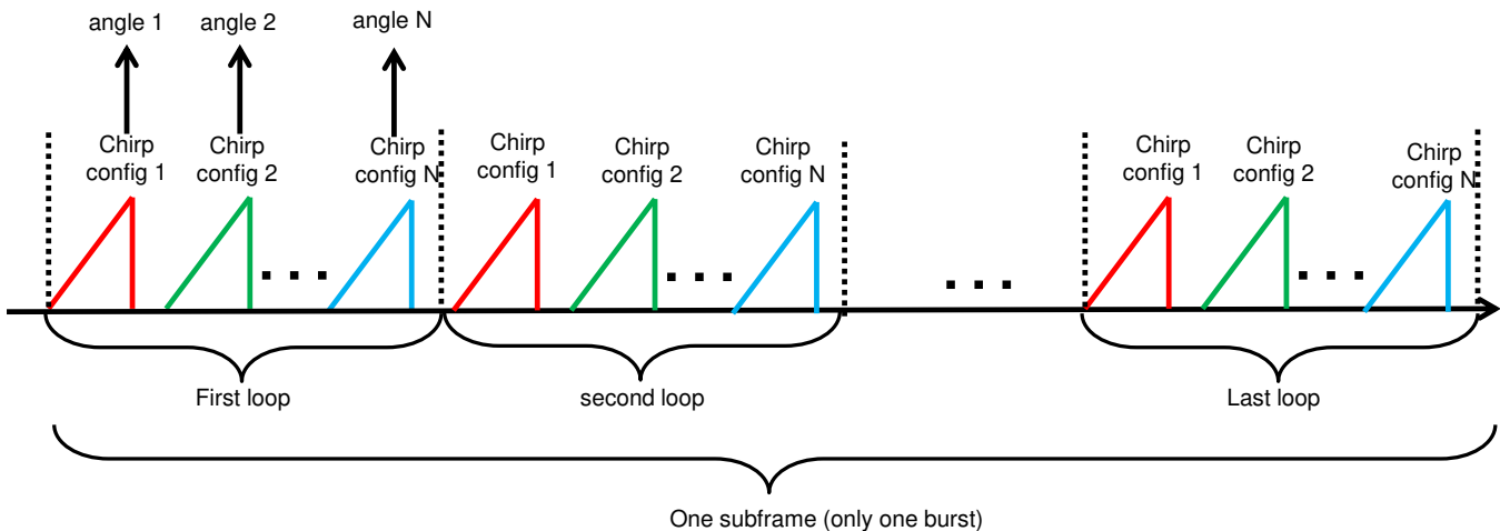
図 10. Chirp Based Beam Steering
