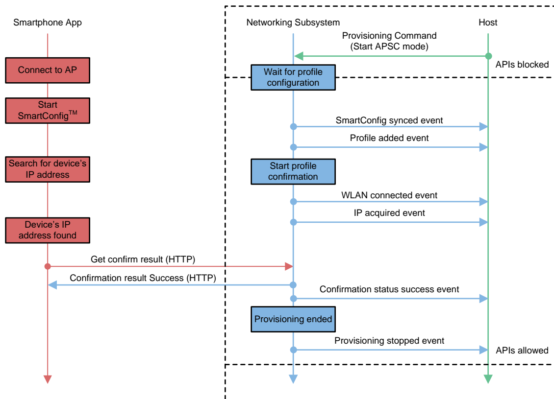
図 7. Timing Diagram for Successful SmartConfig™ Provisioning
