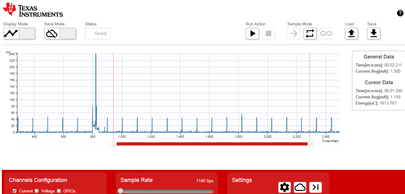
図 16. Current Consumption: Always-Connected Mode During Data Transfer
