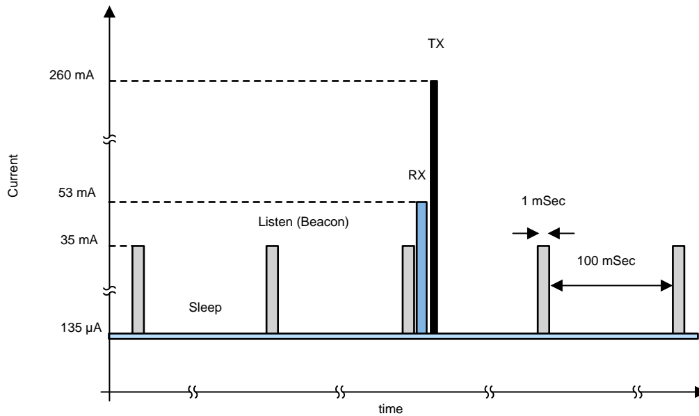
図 8. Current Consumption Pattern in Always-Connected Mode
