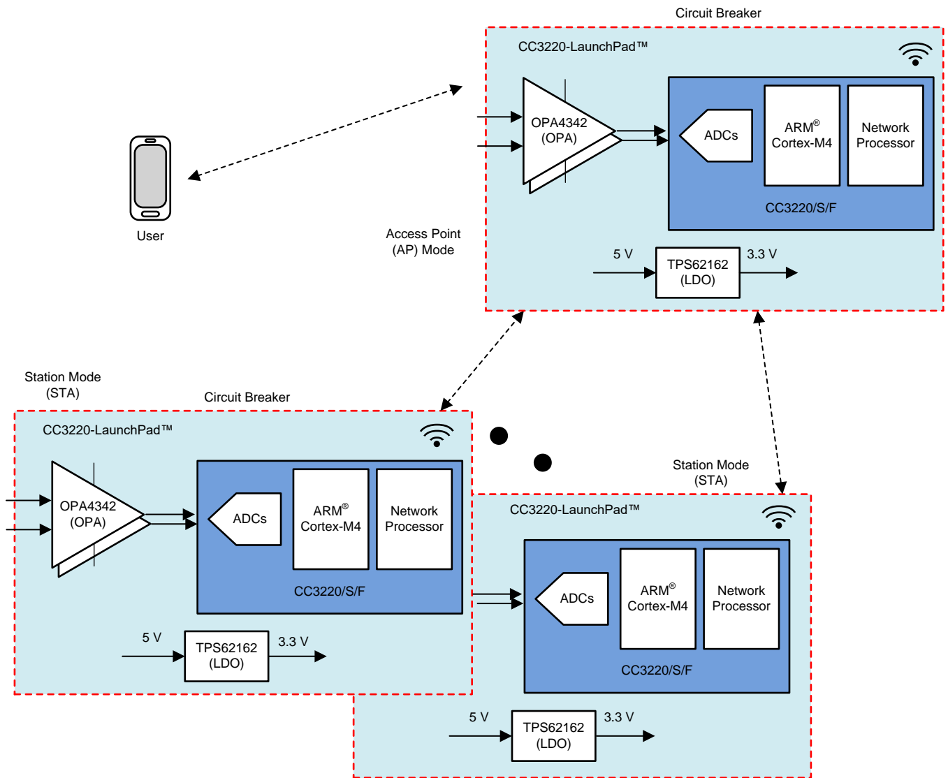
図 6. SimpleLink™ AP Architecture
