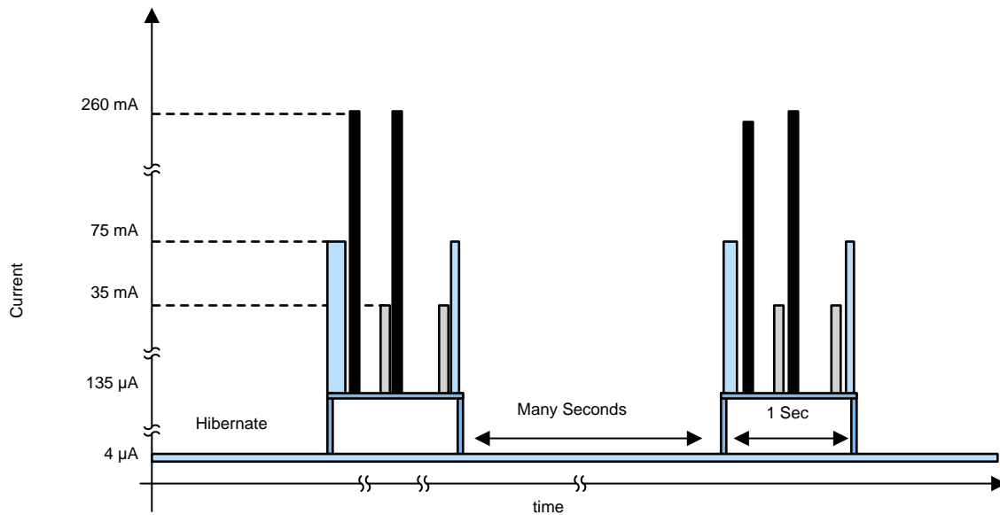
図 9. Current Drawn During Intermittent Connection
