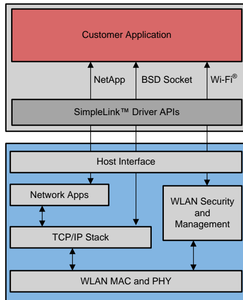
図 4. CC3200x Embedded Software Overview
