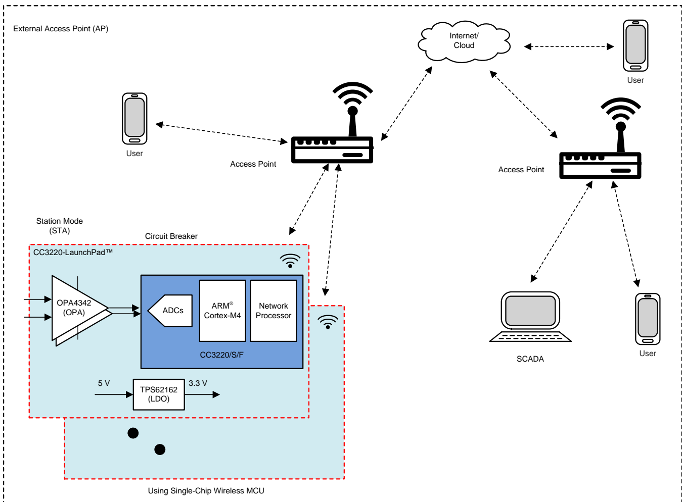
図 5. Wi-Fi® Connectivity Through External Access Point
