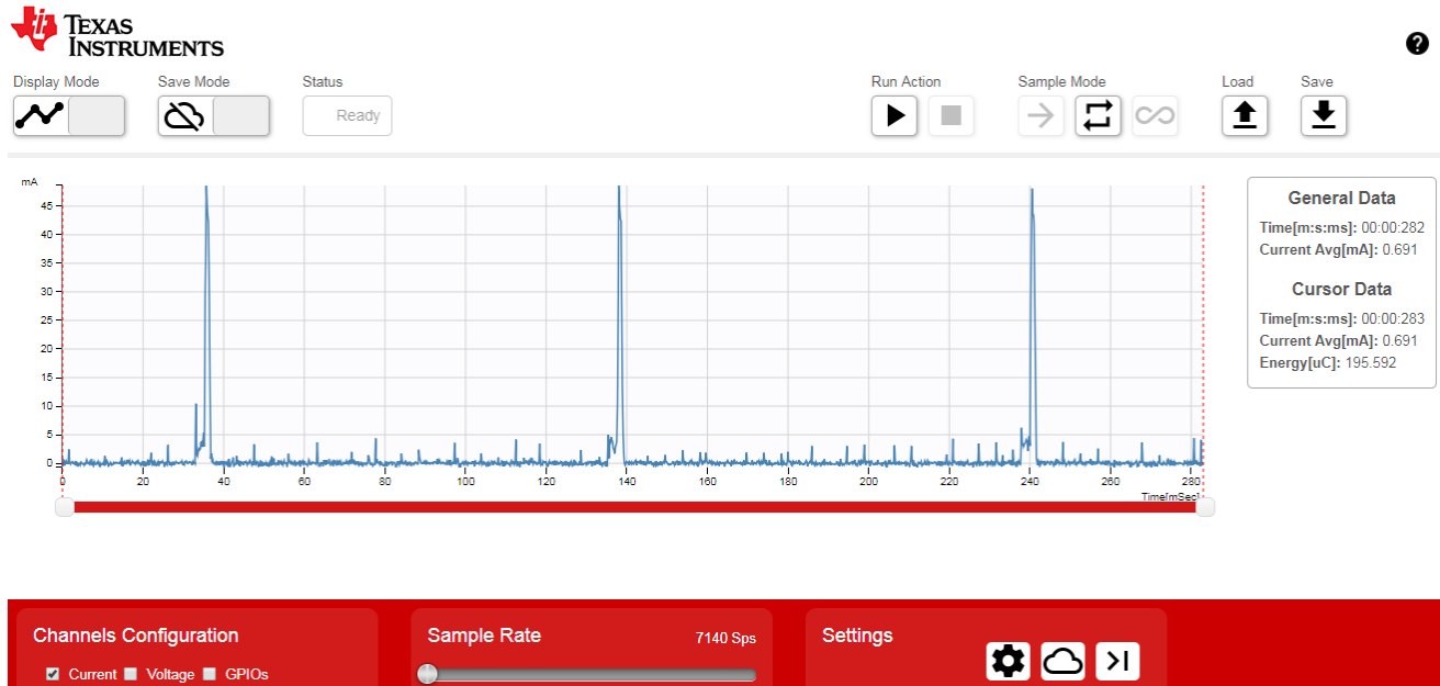
Figure 15. Current Consumption: Always-Connected Mode Without Data Transfer
