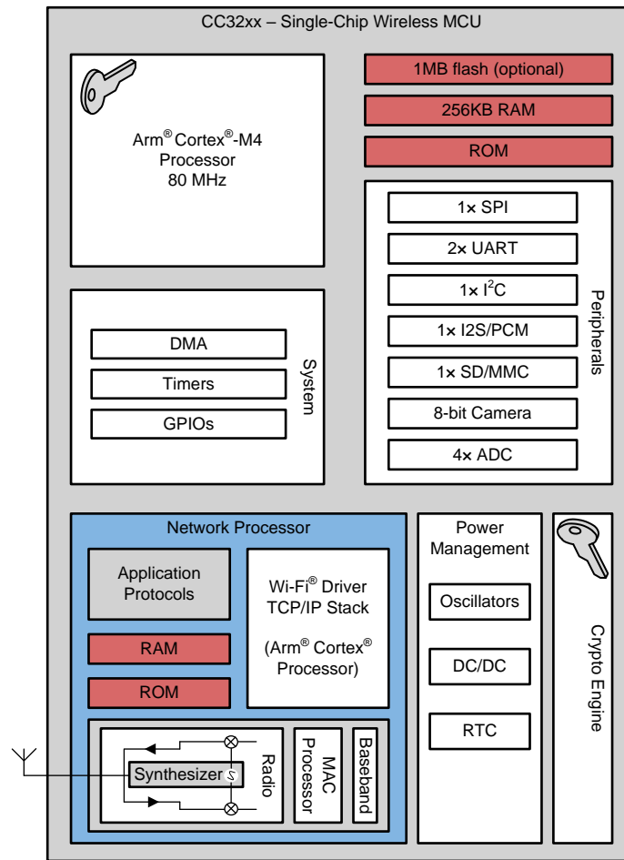
図 3. CC3220X Hardware Overview
