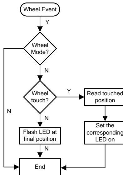
図 7. Wheel Event Flowchart
