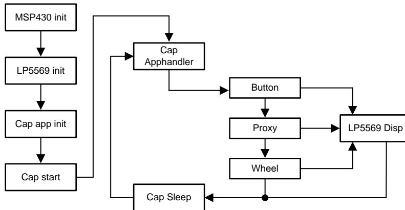
Figure 10. TIDA-01559 Overall State Machine
