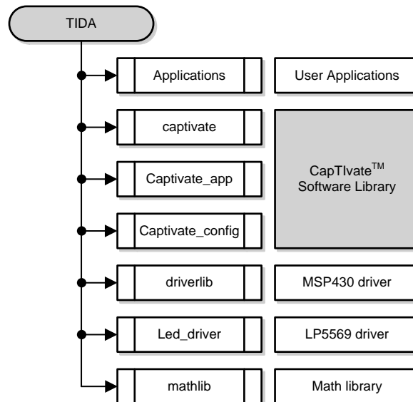
図 4. TIDA-01559 Firmware Structure
