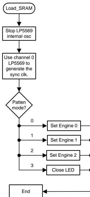
☒ 9. Load SRAM Flowchart
