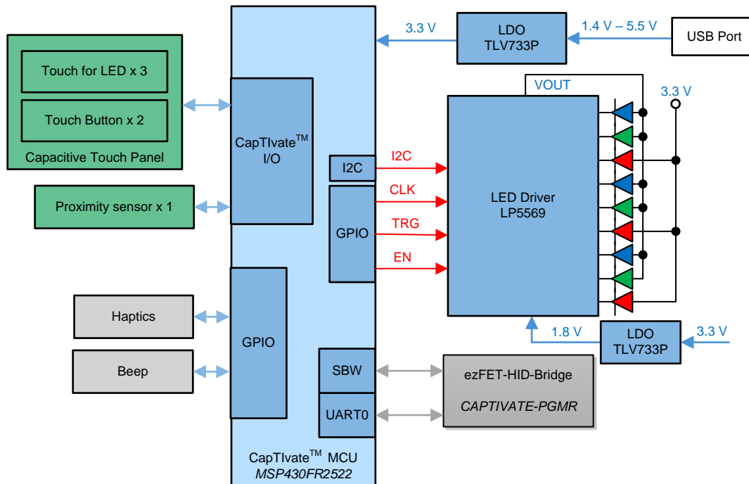
Figure 1. TIDA-01559 Block Diagram
