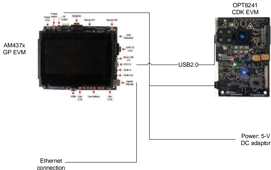
Figure 15. Hardware Setup
