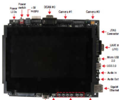
図 7. AM437x GP EVM Top View
