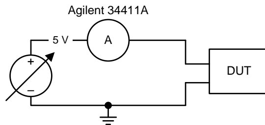
Figure 21. Test Circuit Used for Measuring Supply Current
