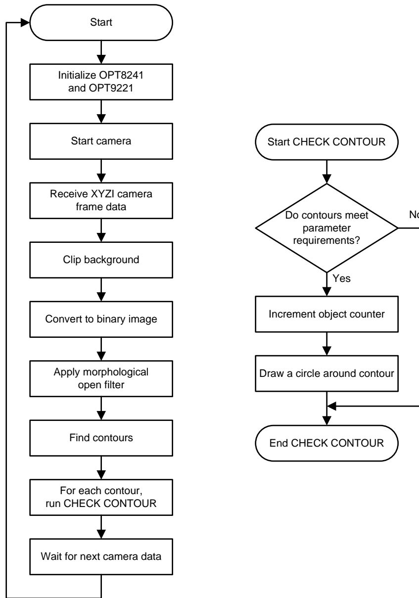
図 20. Simple People Tracking Algorithm Flow Chart
