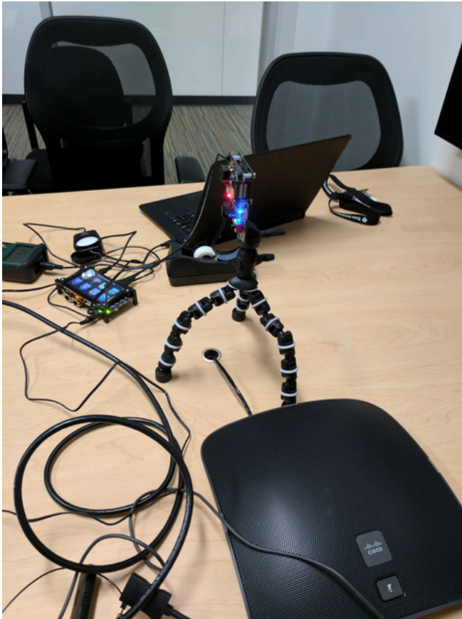
☒ 23. OPT8241 CDK and AM437x GP EVM With Tripod
