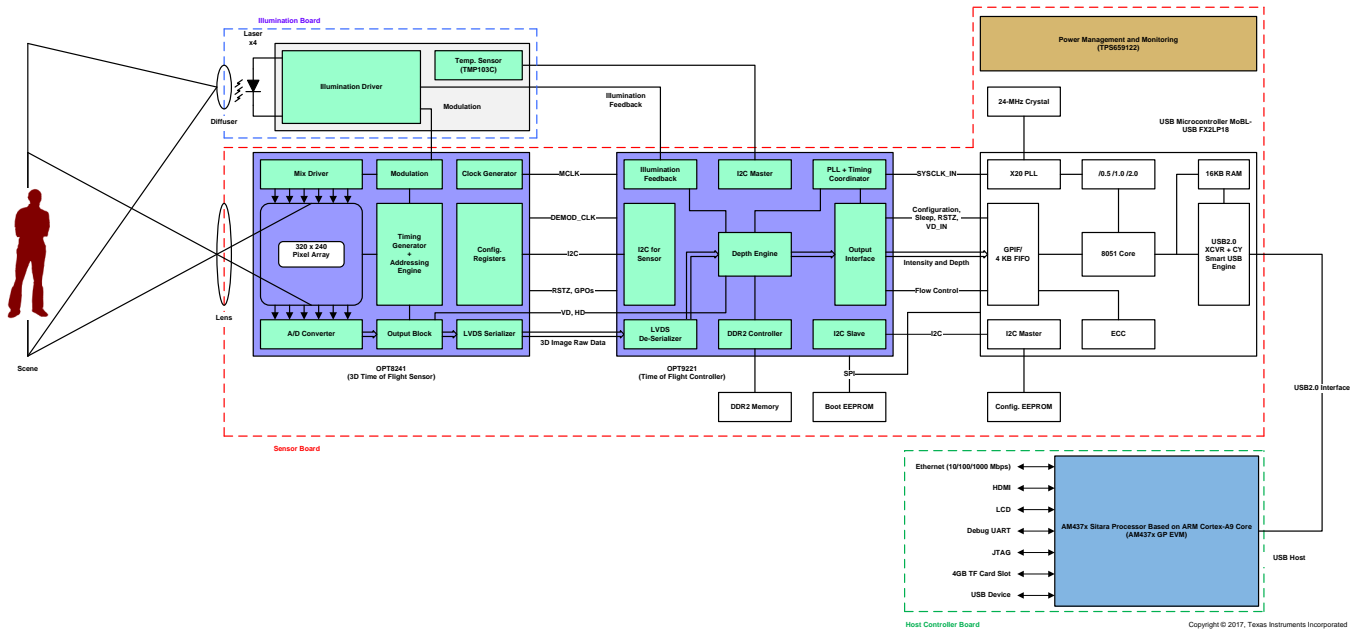
Figure 1. Block Diagram of TIDA-01436
