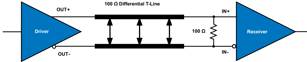
FIG 10-2. Point-to-Point Topology
