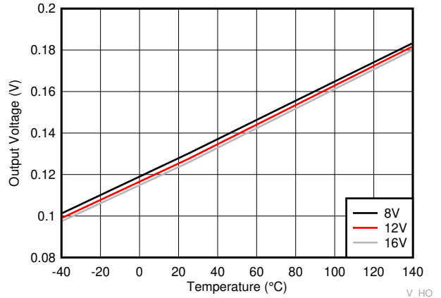
6-15. HO High Output Voltage ( V_{\text{HOH}} )
