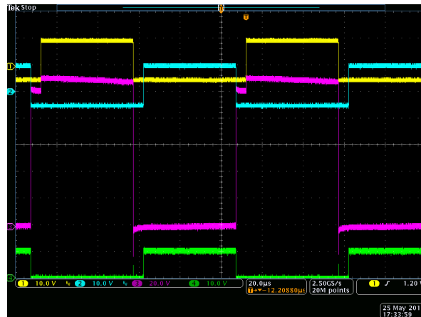
8-7. Propagation Delay and Delay Matching
