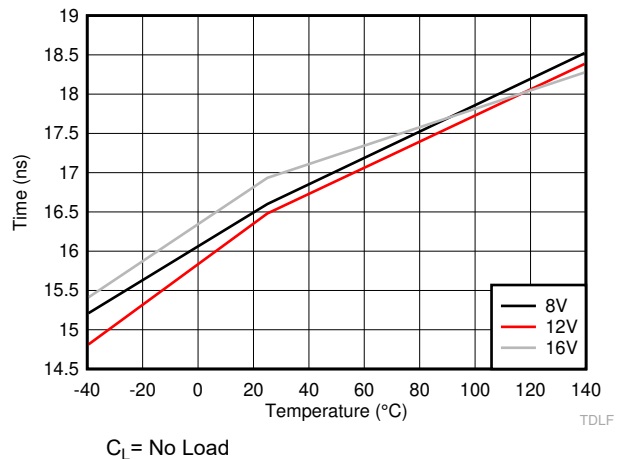
6-25. LO Falling Propagation Delay (TDLFF)
