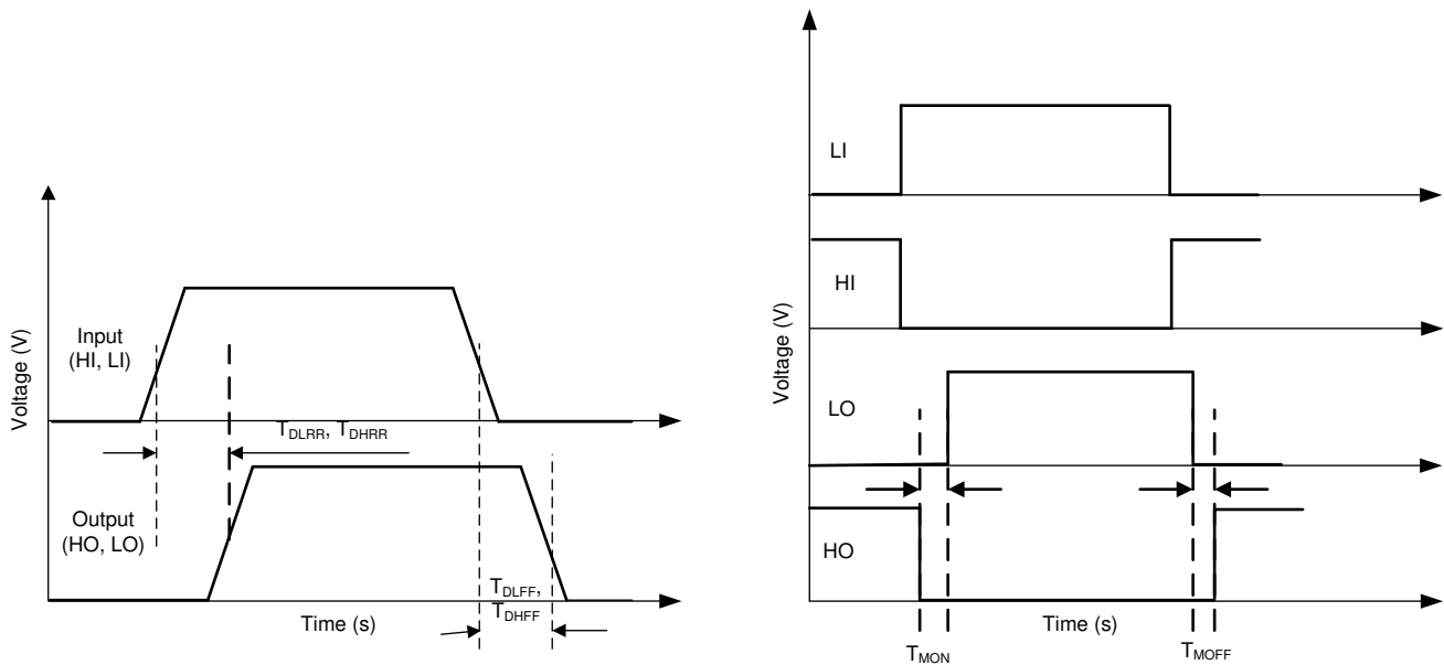
6-1. Timing Diagram
