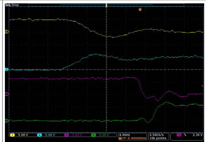
8-8. Propagation Delay and Delay Matching
