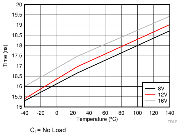
6-24. LO Rising Propagation Delay (TDLRR)
