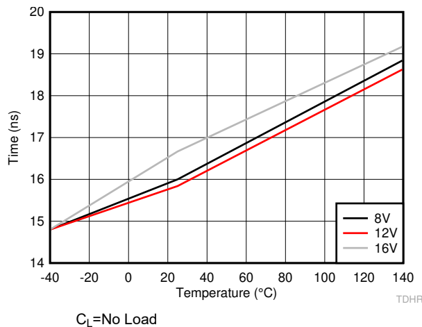
6-22. HO Rising Propagation Delay (TDHRR)
