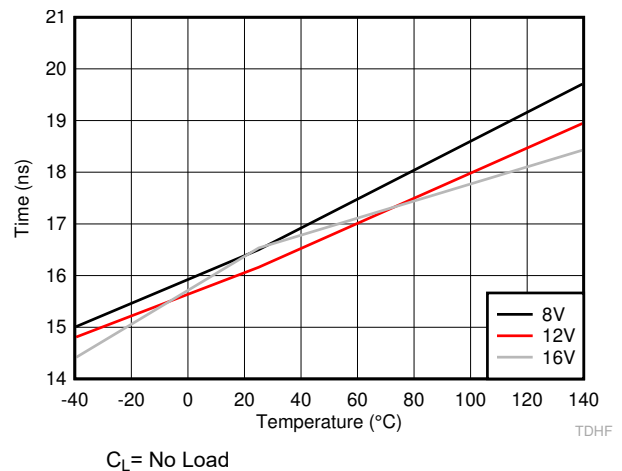
6-23. HO Falling Propagation Delay (TDHFF)
