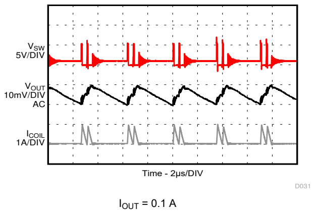
9-13. PSM Operation
