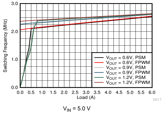
9-8. Switching Frequency
