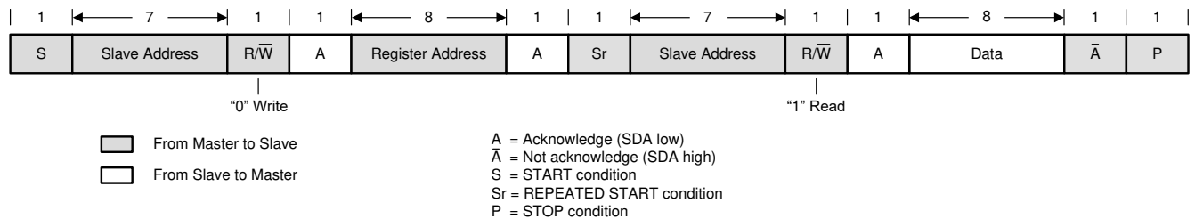
✎ 8-7. “Read” Data Transfer Format in Standard-, Fast, and Fast-Plus Modes
