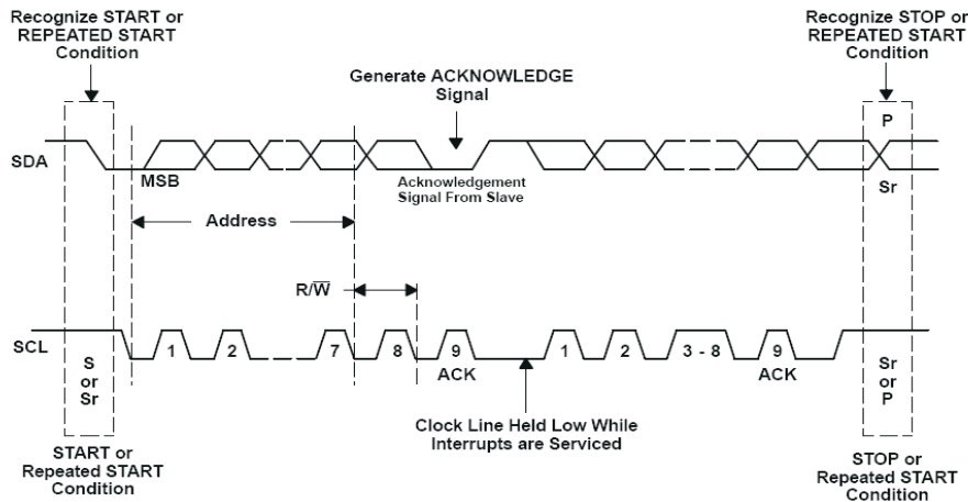
8-5. Bus Protocol
