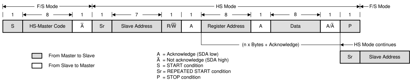
✎ 8-8. Data Transfer Format in HS-Mode
