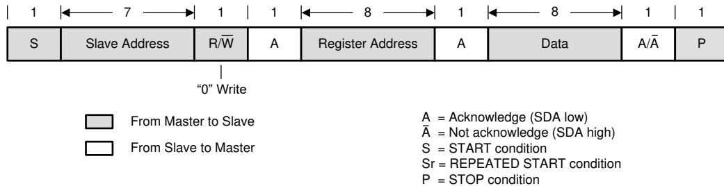
✎ 8-6. “Write” Data Transfer Format in Standard-, Fast, and Fast-Plus Modes
