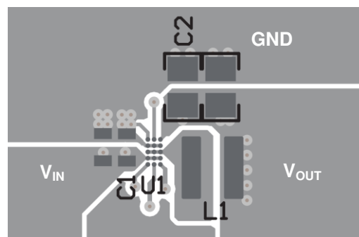
Figure 11-1. Layout Example
