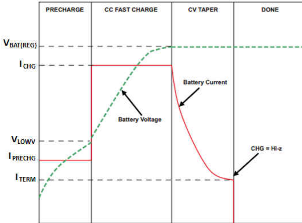
図 9-2. BQ25150 Typical Charge Cycle
