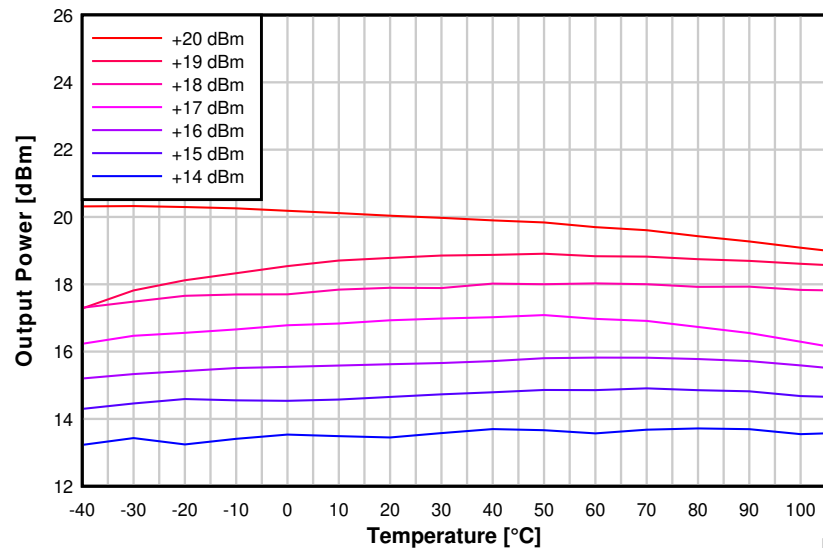
8-40. Output Power vs. Temperature (50 kbps, 915 MHz)
