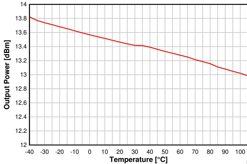
8-39. Output Power vs. Temperature (50 kbps, 868.3 MHz)
