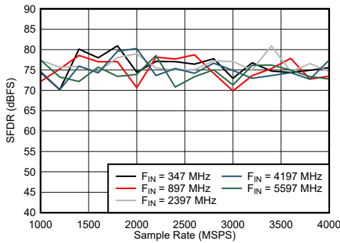
Figure 6-45. Dual Channel Mode: SFDR vs Sample Rate and Input Frequency
