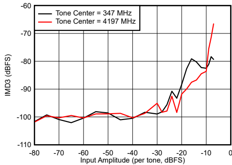
6-107. Dual Channel Mode: IMD3 vs Input Amplitude
