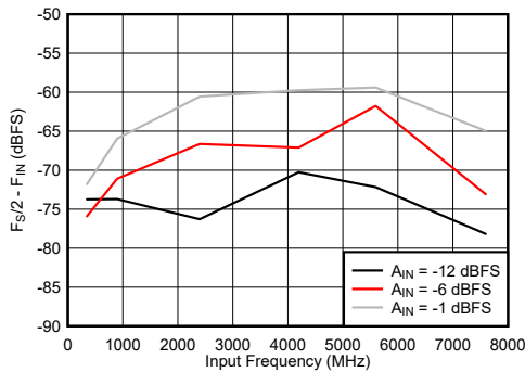
Figure 6-81. DES Mode: F_{\text{S}}/2 - F_{\text{IN}} vs Input Frequency
