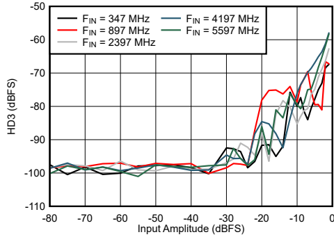
6-61. DES Mode: HD3 vs Input Amplitude and Frequency
