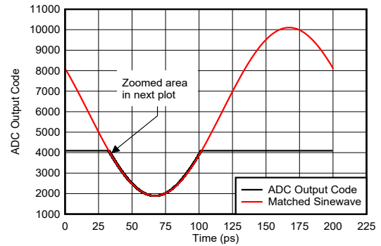
6-143. Sinewave Overdrive Recovery
