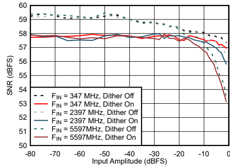
6-56. DES Mode: SNR vs Input Amplitude and Dither
