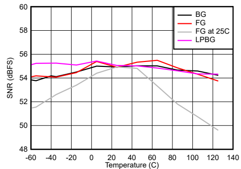
Figure 6-94. Dual Channel Mode: SNR, SINAD and SFDR vs Temperature FG calibration at each temperature
