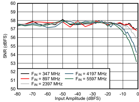
6-67. Dual Channel Mode: SNR vs Input Amplitude and Frequency
