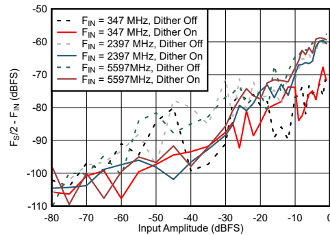
6-64. DES Mode: F_{S/2} - F_{\text{IN}} vs Input Amplitude and Dither
