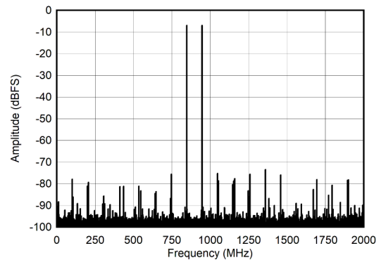
6-24. Dual Channel Mode: Two Tone FFT at 897 MHz
