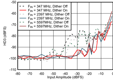
6-62. DES Mode: HD3 vs Input Amplitude and Dither
