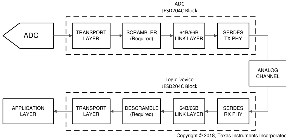
図 7-20. Simplified 64B/66B Encoded JESD204C Interface Diagram
