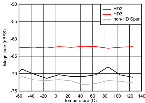
Figure 6-93. DES Mode: HD2, HD3 and Worst non-HD Spur vs Temperature FG calibration at each temperature
