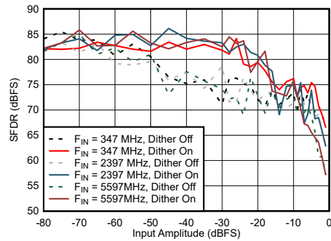
6-70. Dual Channel Mode: SFDR vs Input Amplitude and Dither
