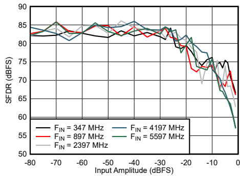
6-69. Dual Channel Mode: SFDR vs Input Amplitude and Frequency
