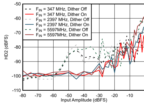
6-72. Dual Channel Mode: HD2 vs Input Amplitude and Dither
