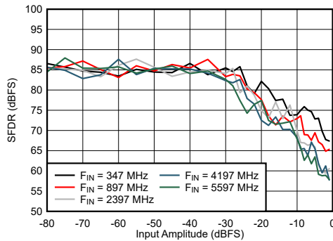
6-57. DES Mode: SFDR vs Input Amplitude and Frequency
