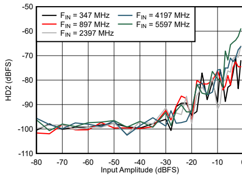
6-71. Dual Channel Mode: HD2 vs Input Amplitude and Frequency
