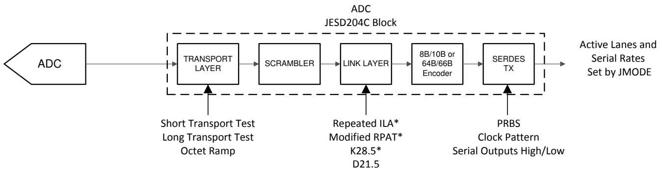
図 7-25. Test Mode Insertion Points
