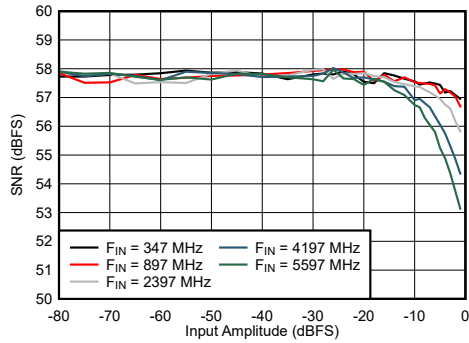
6-55. DES Mode: SNR vs Input Amplitude and Frequency
