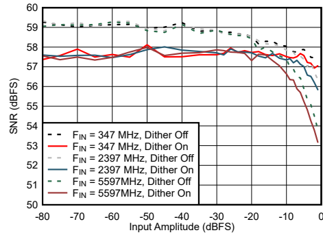
6-68. Dual Channel Mode: SNR vs Input Amplitude and Dither
