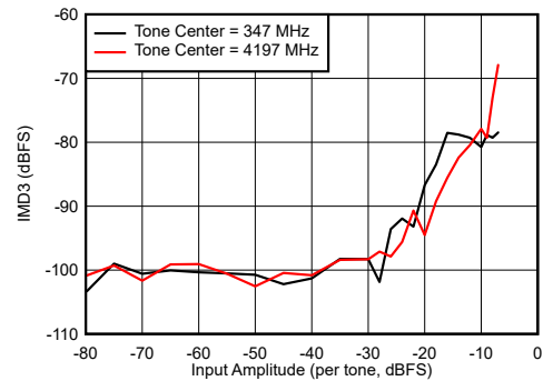
6-106. DES Mode: IMD3 vs Input Amplitude
