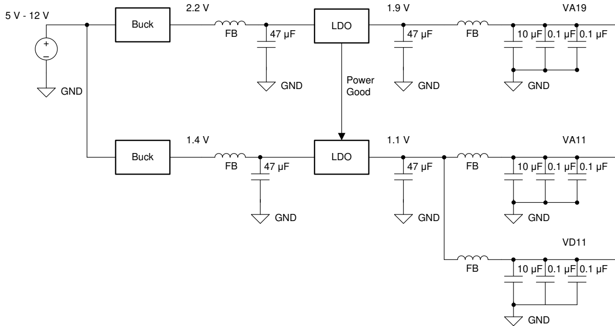
図 8-4. LDO Linear Regulator Approach Example
