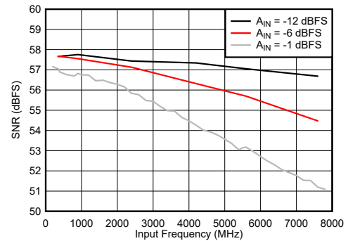
Figure 6-82. DES Mode: F_{\text{IN}} \pm F_{\text{S}}/4 vs Input Frequency
