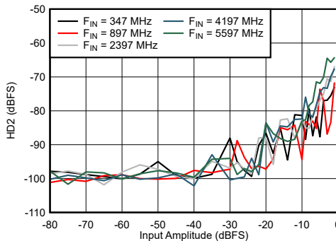
6-59. DES Mode: HD2 vs Input Amplitude and Frequency
