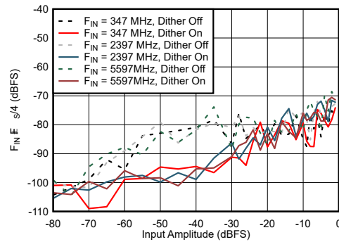
6-66. DES Mode: F_{\text{IN}} \pm F_{\text{IN}/4} vs Input Amplitude and Dither
