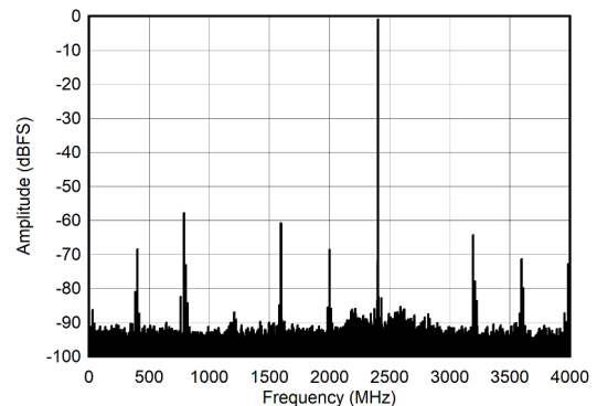
图 6-12. DES Mode: Single Tone FFT at 5597 MHz
