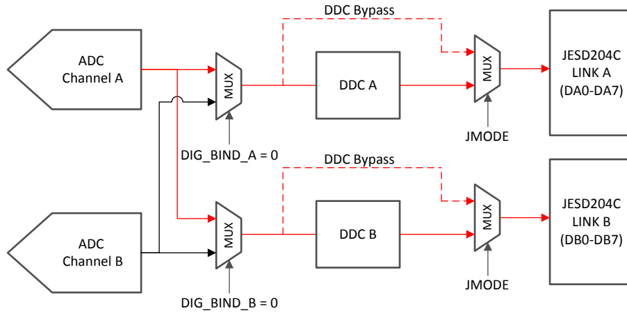
図 7-24. Dual DDC Mode or Redundant Data Mode for Channel A
