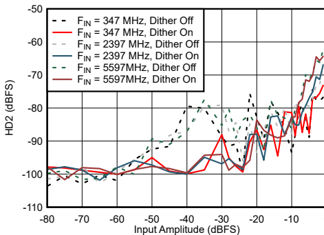
6-60. DES Mode: HD2 vs Input Amplitude and Dither
