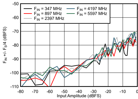
6-65. DES Mode: F_{\text{IN}} \pm F_{S/4} vs Input Amplitude and Frequency
