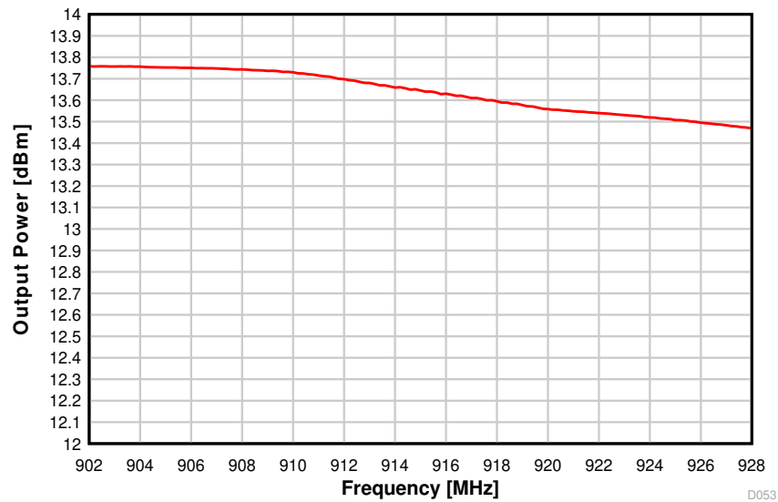
8-40. Output Power vs. Frequency (50 kbps, 915 MHz)
