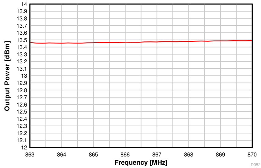
8-39. Output Power vs. Frequency (50 kbps, 868 MHz)
