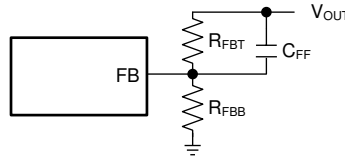
✎ 19. Feed-Forward Capacitor for Loop Compensation
