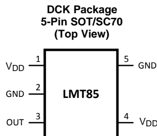
Pin Functions
