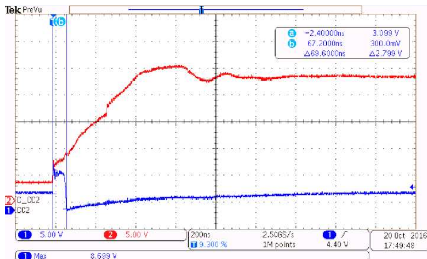
☒ 29. TPD6S300 Protecting the TPS65982 During a Short-to- V_{BUS} Event
