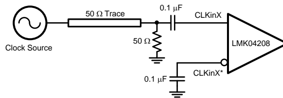
Figure 25. CLKinX/X* Single-Ended Termination
