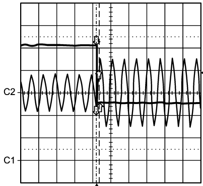
FIGURE 4. Output Signal with the LPV531 Op Amp
