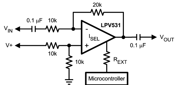
FIGURE 2. AC-Coupled Inverting Amplifier with the LPV531 Amplifier
