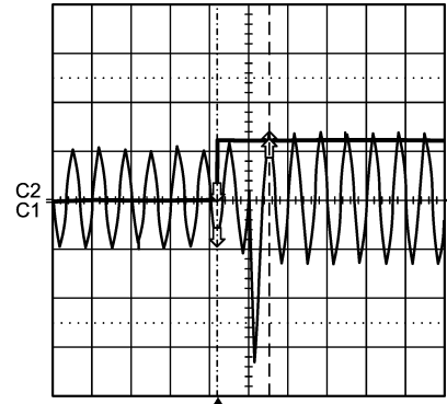
FIGURE 5. Output Signal with an Amplifier with Shutdown
