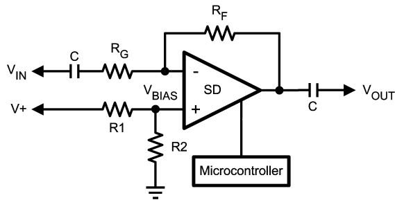
FIGURE 1. AC-Coupled Inverting Amplifier with Shutdown Pin
