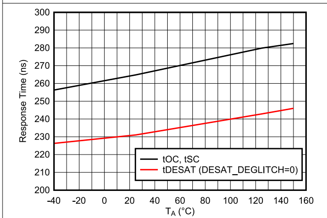
Figure 6-17. Overcurrent Protection Response Time vs. Temperature
