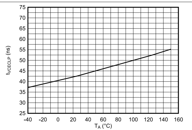
Figure 6-18. VCECLP Intervention Time vs. Temperature
