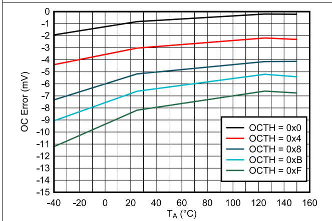
Figure 6-15. OC Threshold Error vs. Temperature
