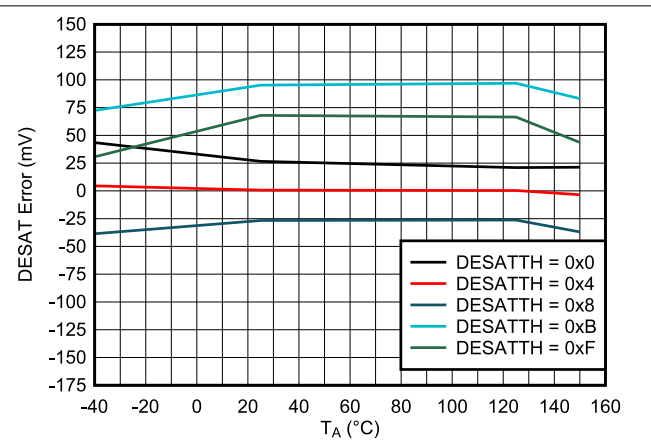
Figure 6-14. DESAT Threshold Error vs. Temperature
