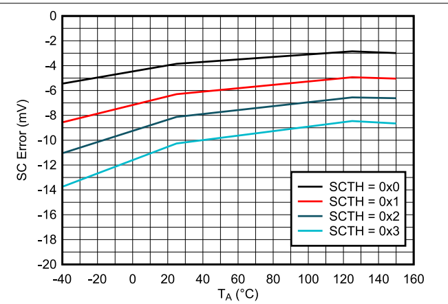
Figure 6-16. SC Threshold Error vs. Temperature
