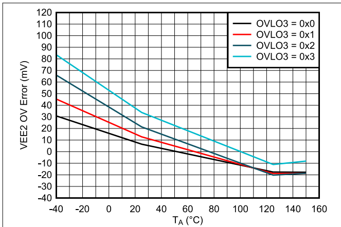
Figure 6-13. VEE2 OVLO Error vs. Temperature
