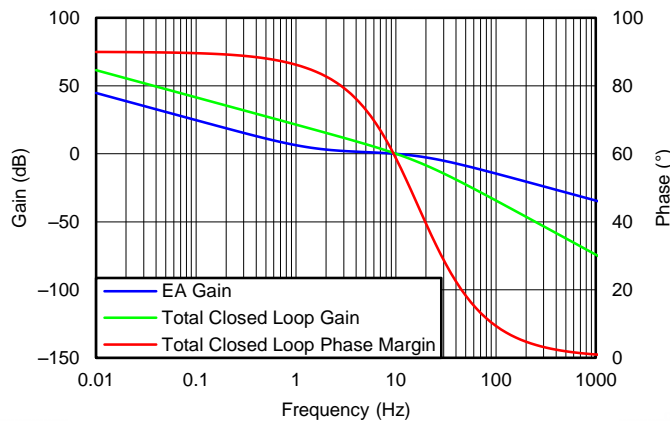
Fig 34. Closed Loop Voltage Bode Plot
