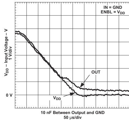
7-20. Output Behavior vs V_{DD} (UCC37321)
