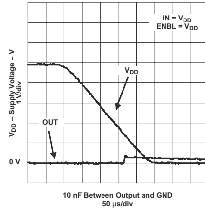
☒ 7-22. Output Behavior vs VDD (Inverting)
