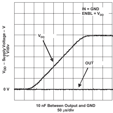
☒ 7-23. Output Behavior vs VDD (Noninverting)
