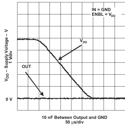
☒ 7-24. Output Behavior vs VDD (Noninverting)
