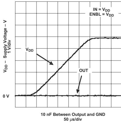
☒ 7-21. Output Behavior vs VDD (Inverting)
