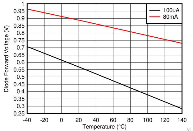
6-16. Boot Diode Forward Voltage Drop
