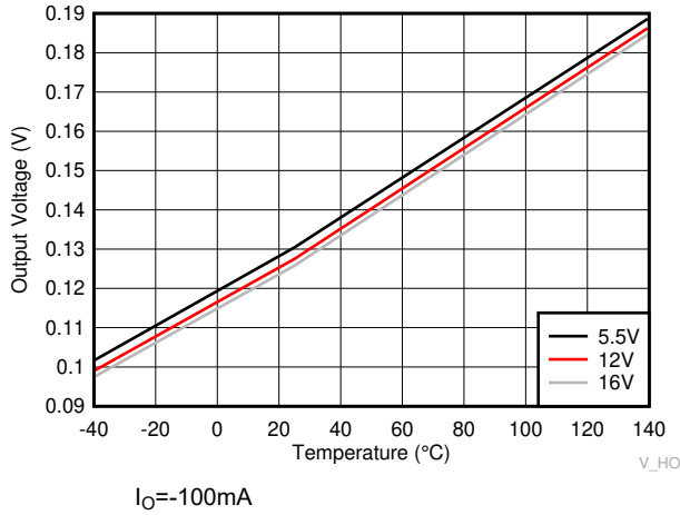
6-21. HO High Output Voltage ( V_{HOH} )
