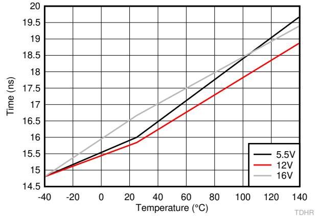
6-28. HO Rising Propagation Delay (TDHR)
