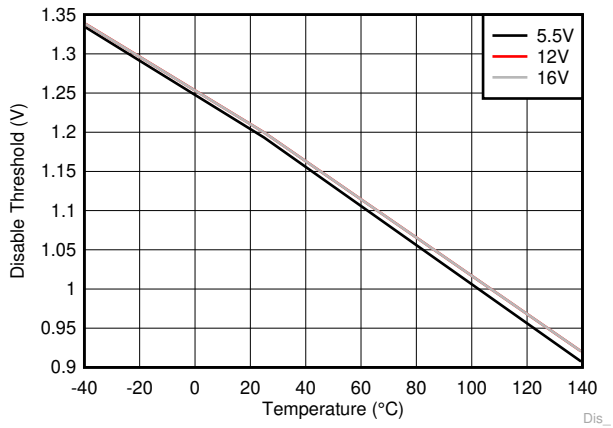
6-11. Disable Threshold
