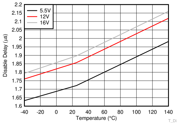
6-13. Disable Delay
