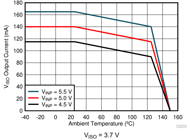
6-11. Maximum V_{ISO} Output Current vs. Temperature
