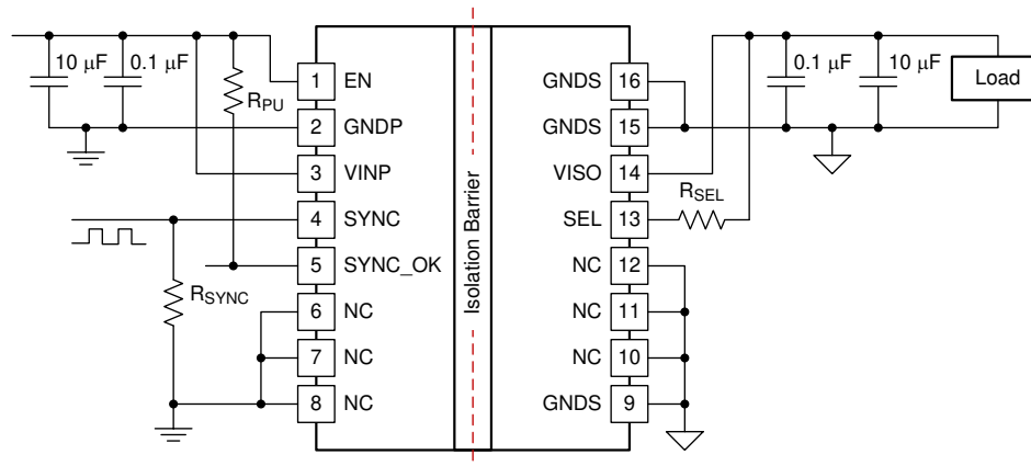
图 8-1. Typical Application
