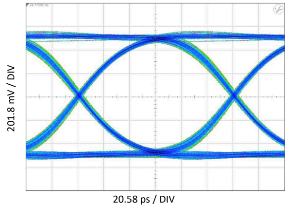
5-12. DisplayPort HBR3 Eye-Pattern Performance with 12in Input PCB Trace at 8.1Gbps
