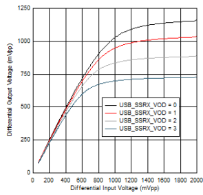
图 5-15. USB SSRX VOD Linearity Settings at 100MHz
