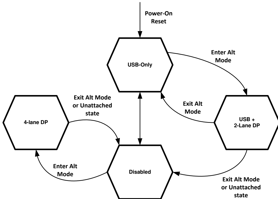
図 6-1. Recommended Mode Transitions
