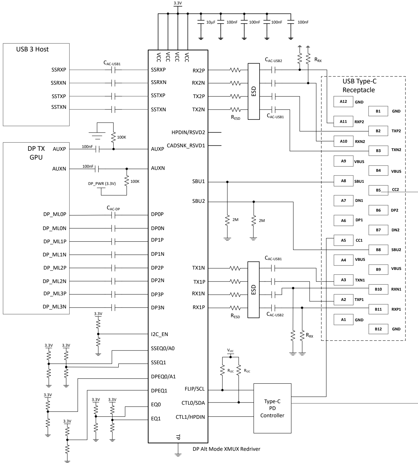
8-2. Application Circuit
