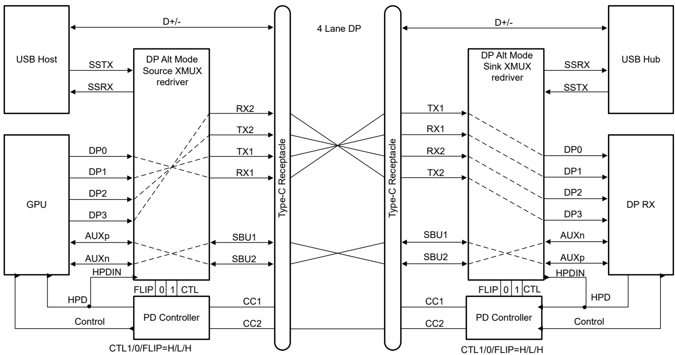
8-9. 4-Lane DP – With Flip (CTL1 = H, CTL0 = L, FLIP = H)
