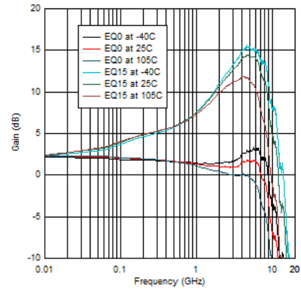
图 5-4. USB RX1 EQ Settings Curves Across Temperature
