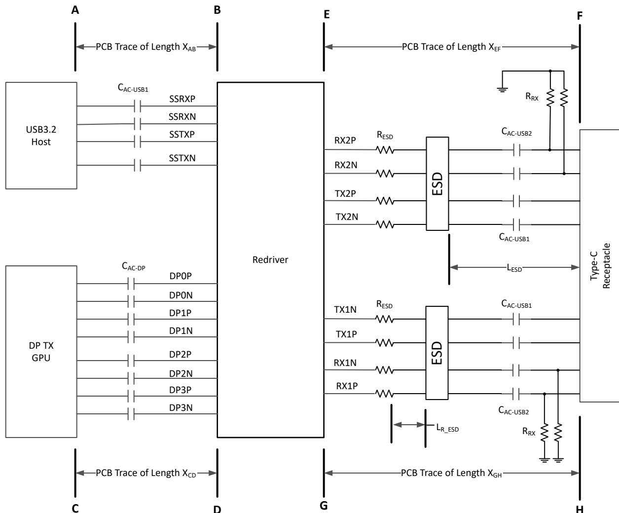
図 8-1. TUSB5461-Q1 in a Host Application
