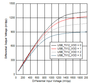
图 5-16. USB TX1 VOD Linearity Settings at 100MHz
