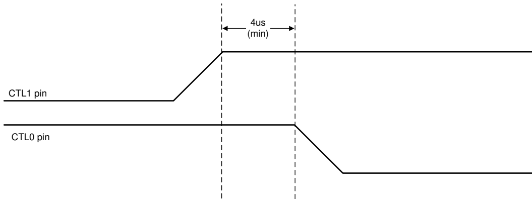
图 6-2. USB to 4-Lane DisplayPort in GPIO Mode
