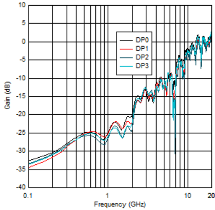
5-9. DisplayPort Input Return Loss Performance
