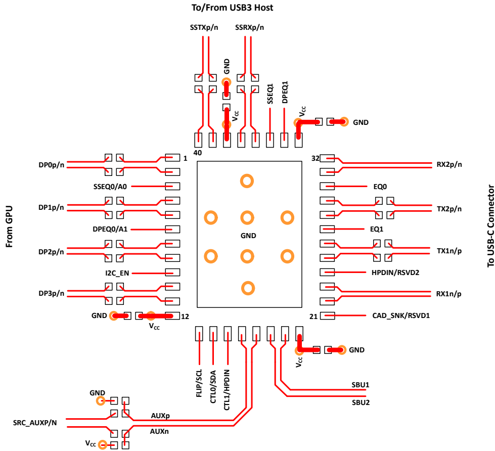
8-10. Layout Example
