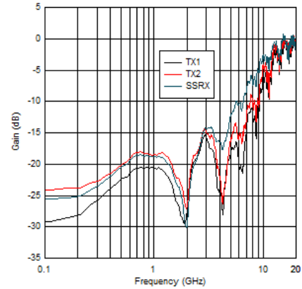
5-10. USB Output Return Loss Performance
