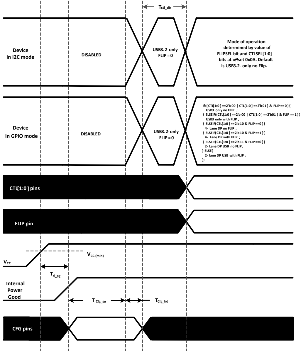
図 6-10. Power-On Timing
