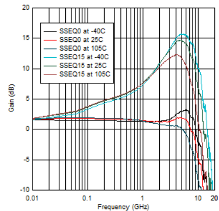
图 5-6. USB SSTX EQ Settings Curves Across Temperature
