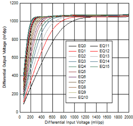
5-7. DisplayPort Linearity Curves at 4.05GHz
