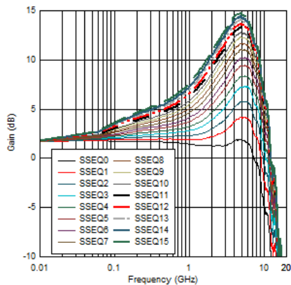
图 5-5. USB SSTX EQ Settings Curves
