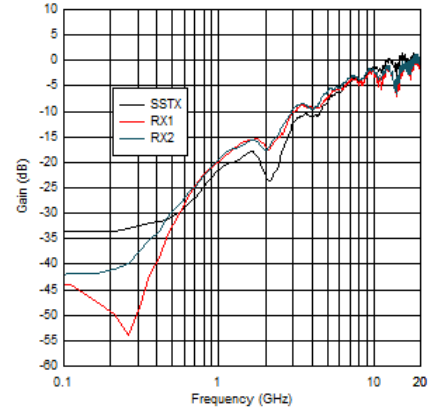
5-8. USB Input Return Loss Performance
